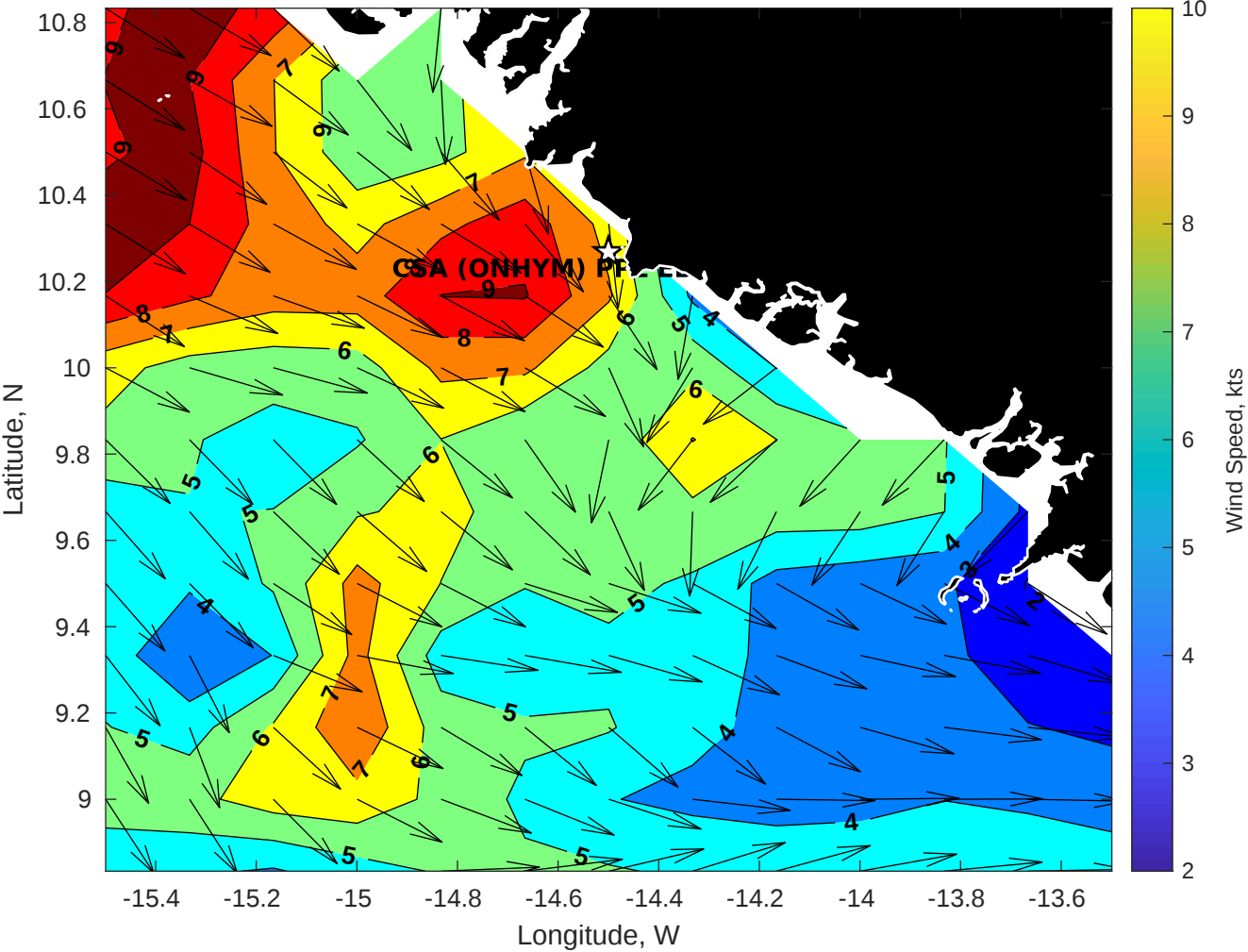
Winds (kts) for CSA (ONHYM) PPL EBS - Guinea at 06-Nov-2025 09:00:00
