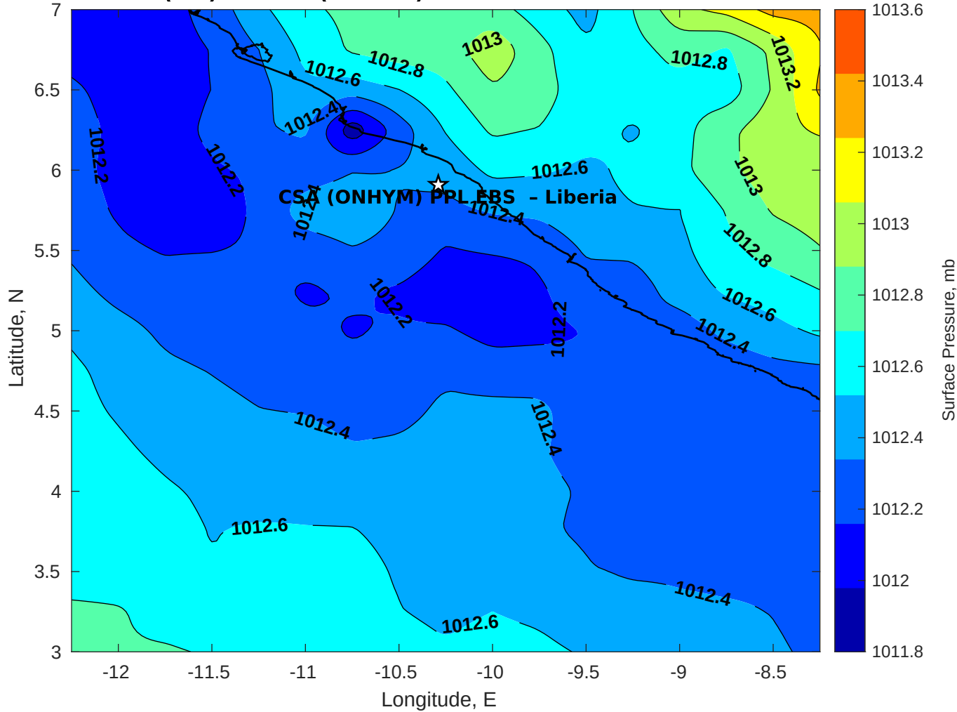
Surface Pressure (mb) for CSA (ONHYM) PPL EBS - Liberia at 07-Nov-2025 00:00:00
