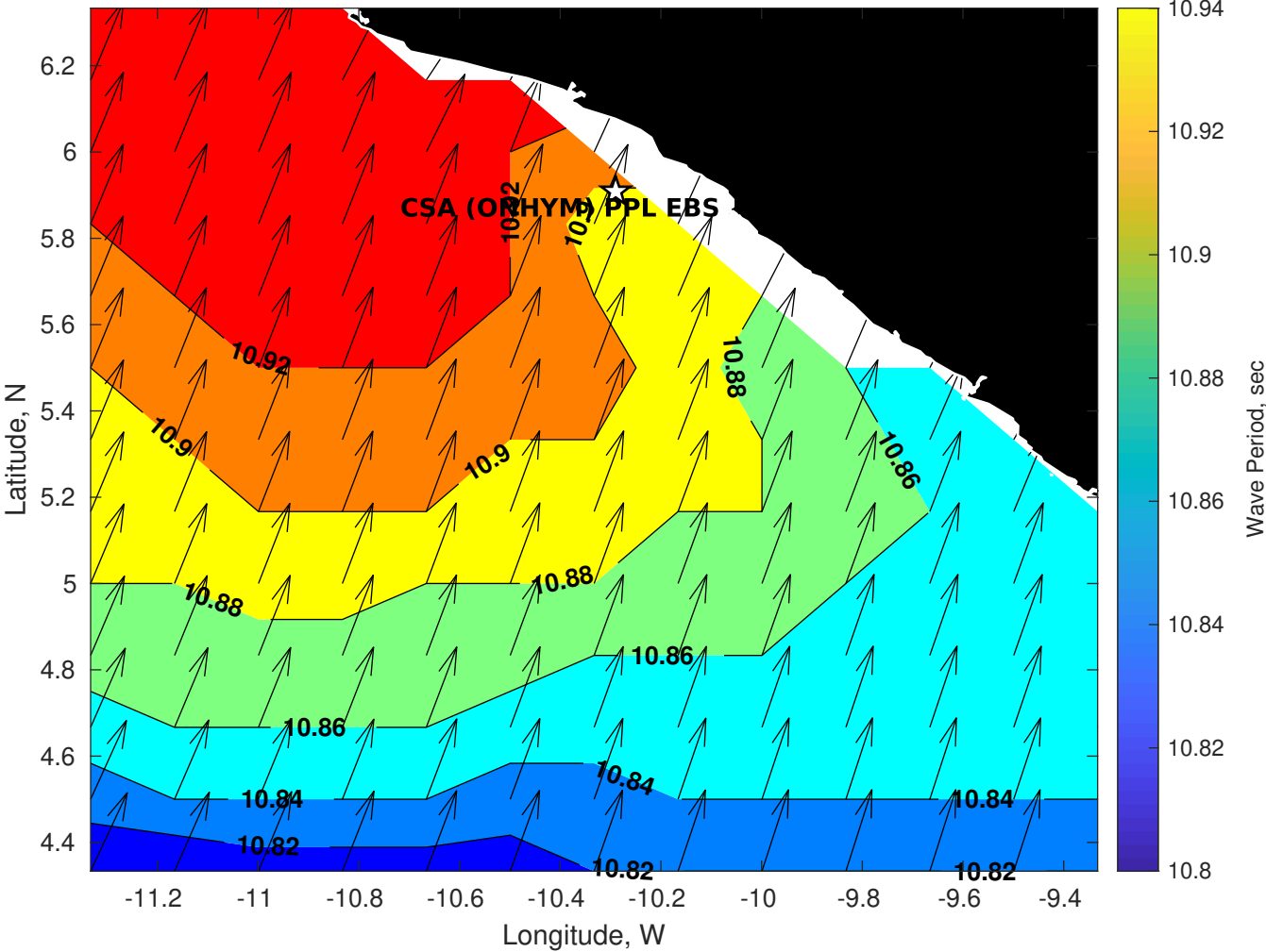
Wave Period (sec) for CSA (ONHYM) PPL EBS - Liberia at 06-Nov-2025 09:00:00
