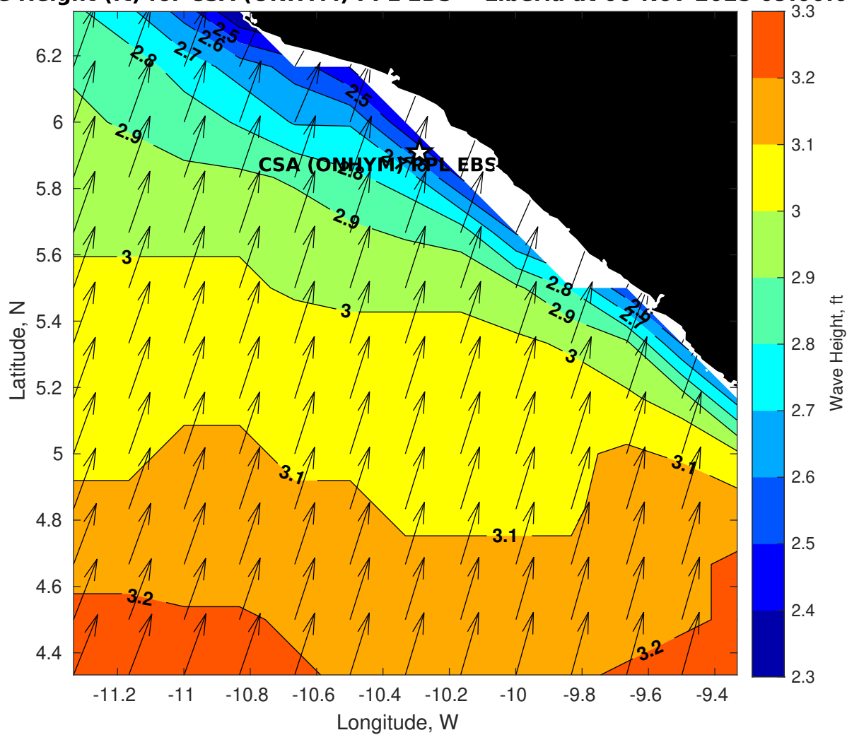
Wave Height (ft) for CSA (ONHYM) PPL EBS - Liberia at 06-Nov-2025 09:00:00
