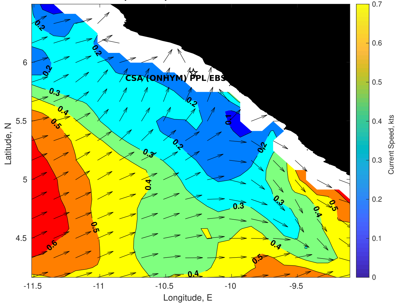
Surface Currents for CSA (ONHYM) PPL EBS - Liberia at 05-Nov-2025 00:00:00
