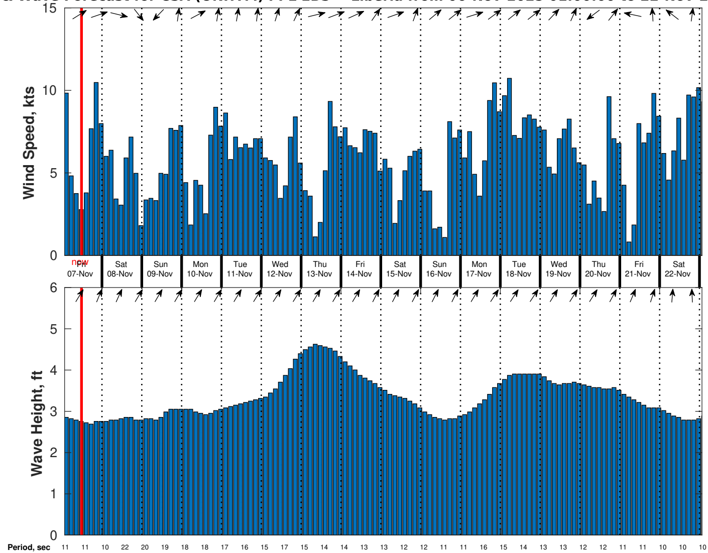
Wind & Wave Forecast for CSA (ONHYM) PPL EBS - Liberia from 06-Nov-2025 01:00:00 to 22-Nov-2025 01:00:00
