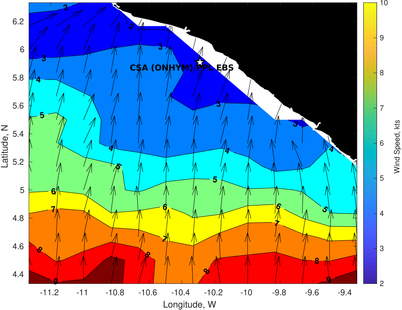
Winds (kts) for CSA (ONHYM) PPL EBS - Liberia at 06-Nov-2025 09:00:00
