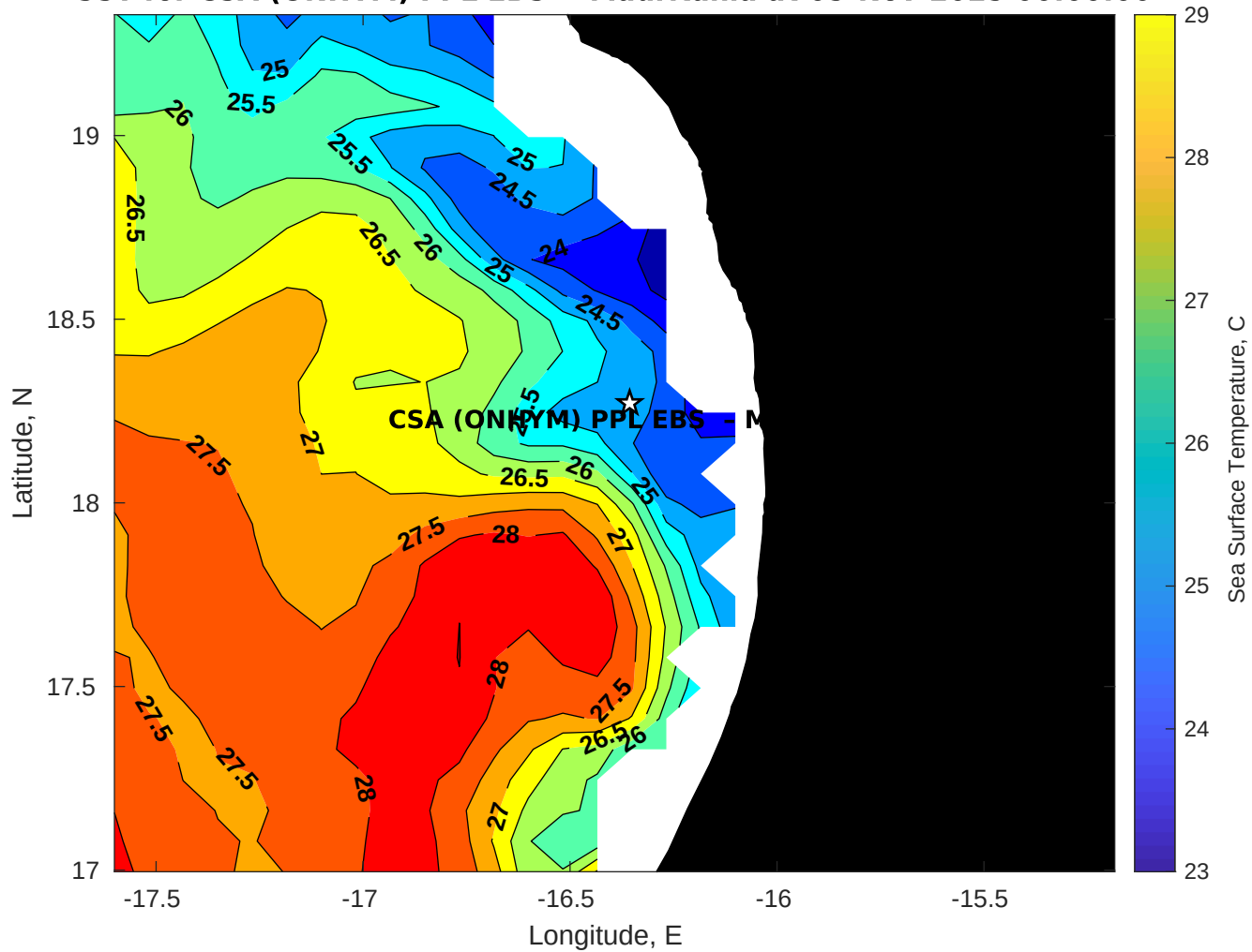
SST for CSA (ONHYM) PPL EBS - Mauritania at 05-Nov-2025 00:00:00
