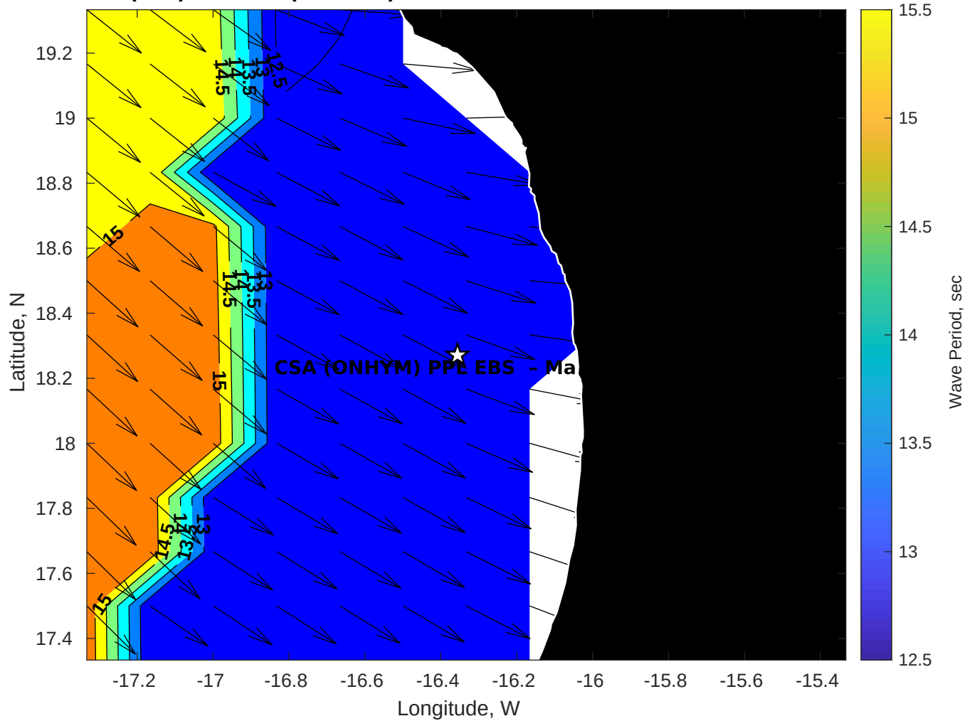
Wave Period (sec) for CSA (ONHYM) PPL EBS - Mauritania at 06-Nov-2025 09:00:00
