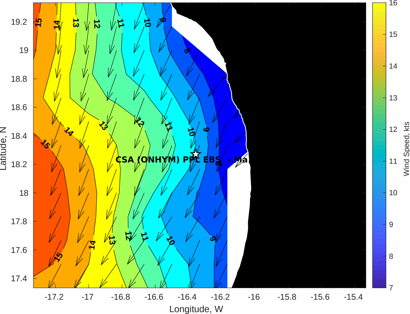
Winds (kts) for CSA (ONHYM) PPL EBS - Mauritania at 06-Nov-2025 09:00:00
