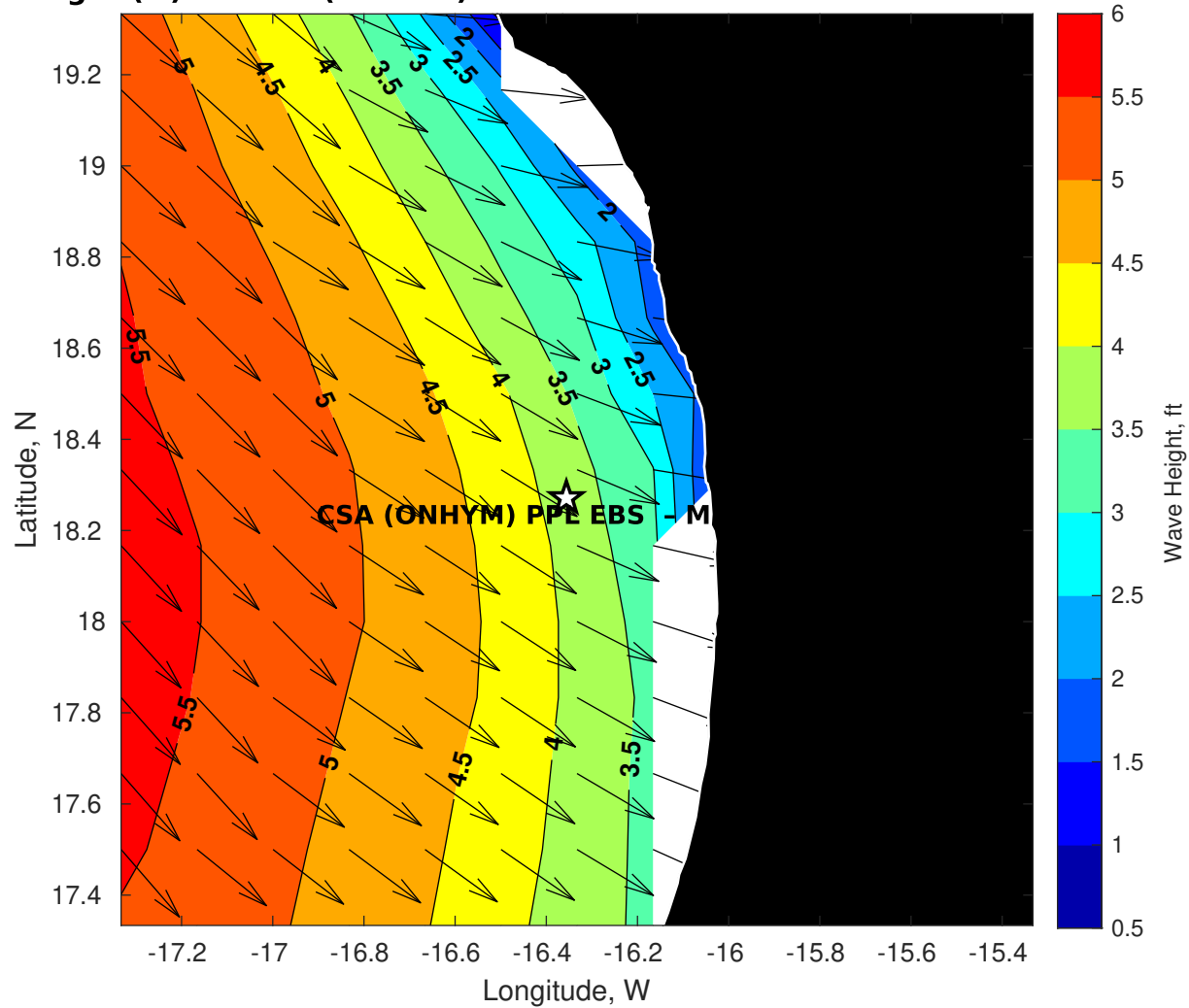
Wave Height (ft) for CSA (ONHYM) PPL EBS - Mauritania at 06-Nov-2025 09:00:00
