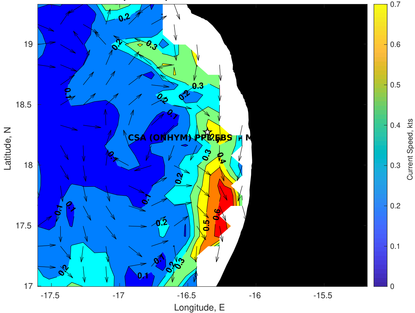
Surface Currents for CSA (ONHYM) PPL EBS - Mauritania at 05-Nov-2025 00:00:00
