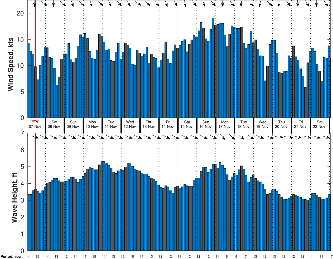
Wind & Wave Forecast for CSA (ONHYM) PPL EBS - Mauritania from 06-Nov-2025 01:00:00 to 22-Nov-2025 01:00:00
