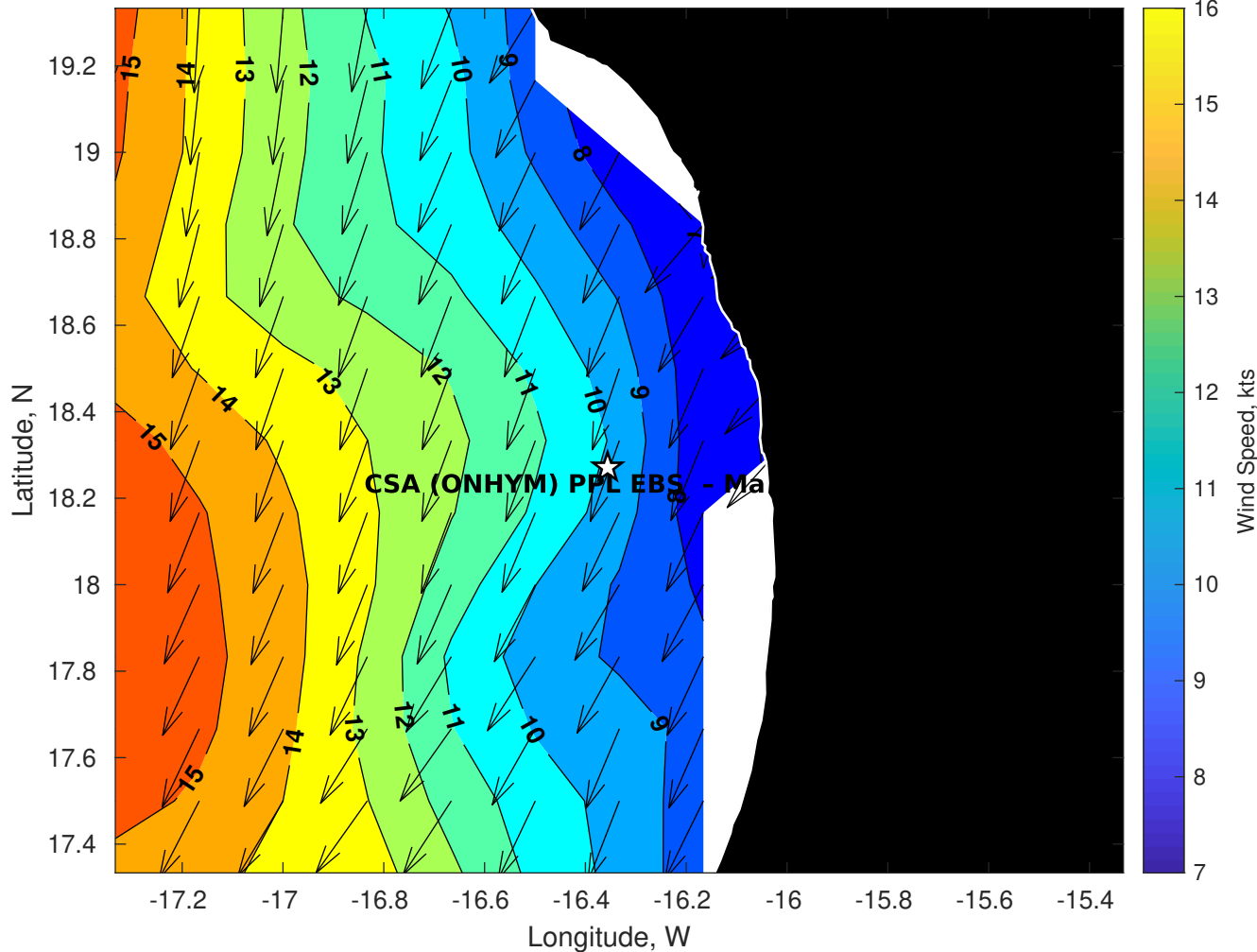
Winds (kts) for CSA (ONHYM) PPL EBS - Mauritania at 06-Nov-2025 09:00:00
