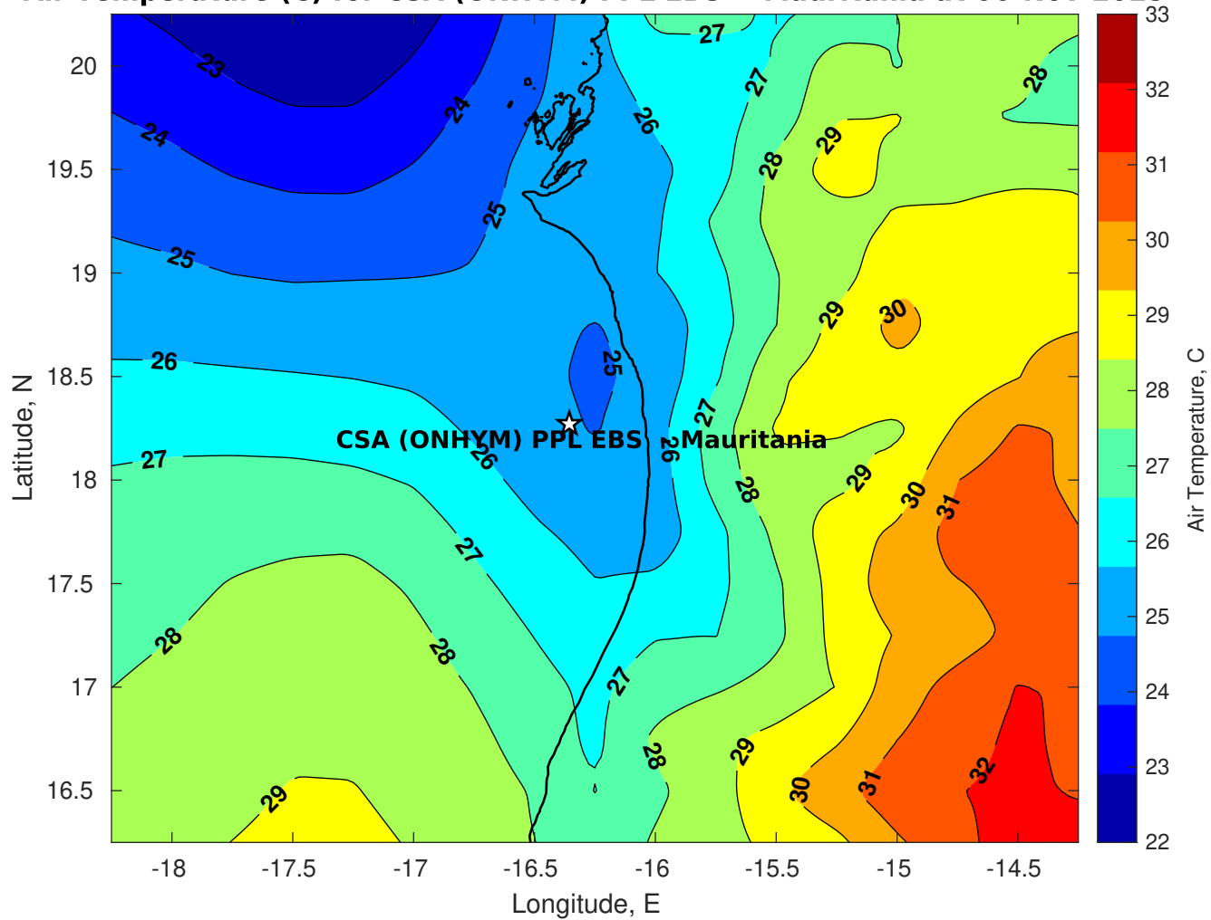
Air Temperature (C) for CSA (ONHYM) PPL EBS - Mauritania at 06-Nov-2025
