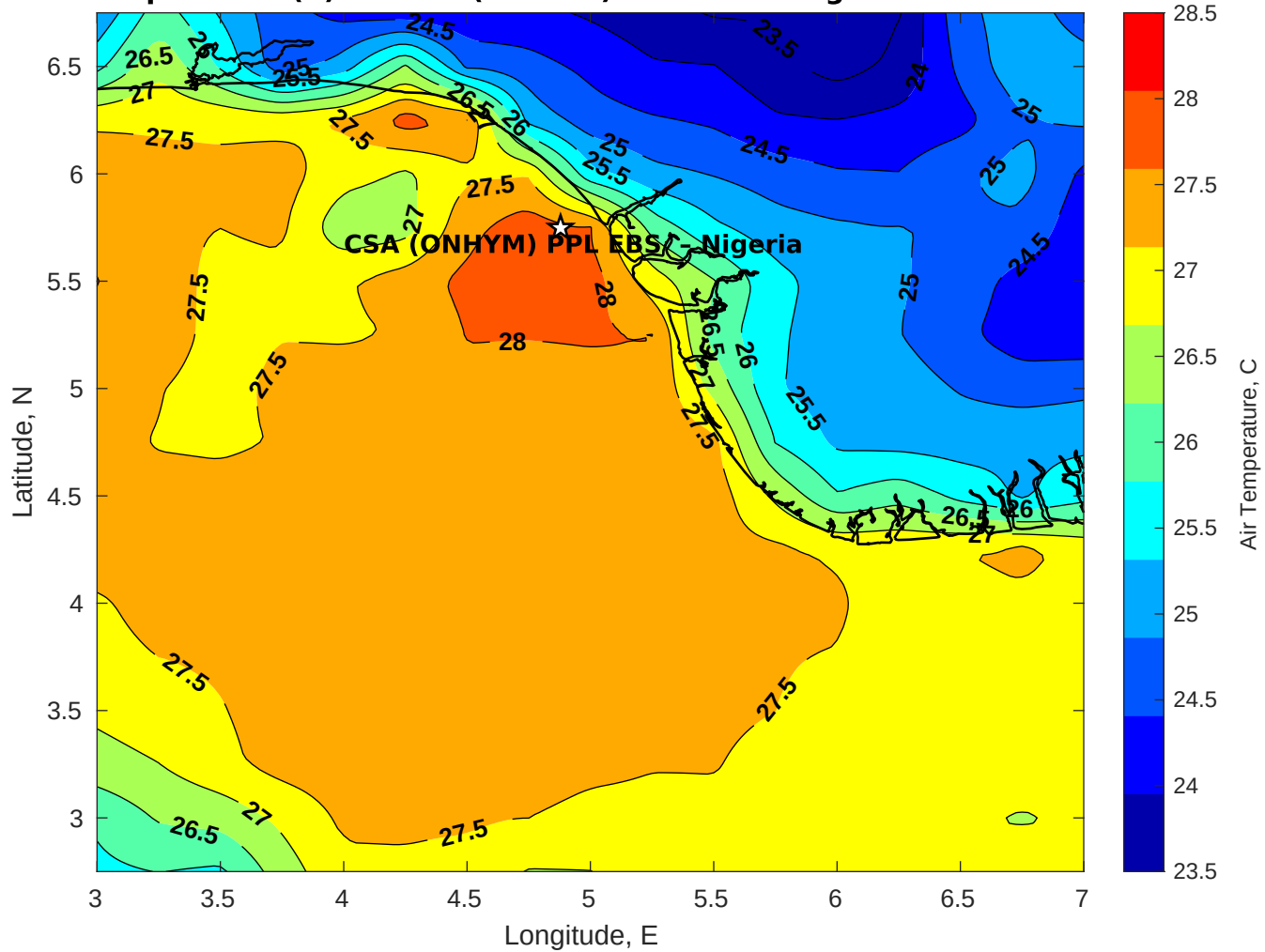
Air Temperature (C) for CSA (ONHYM) PPL EBS - Nigeria at 06-Nov-2025
