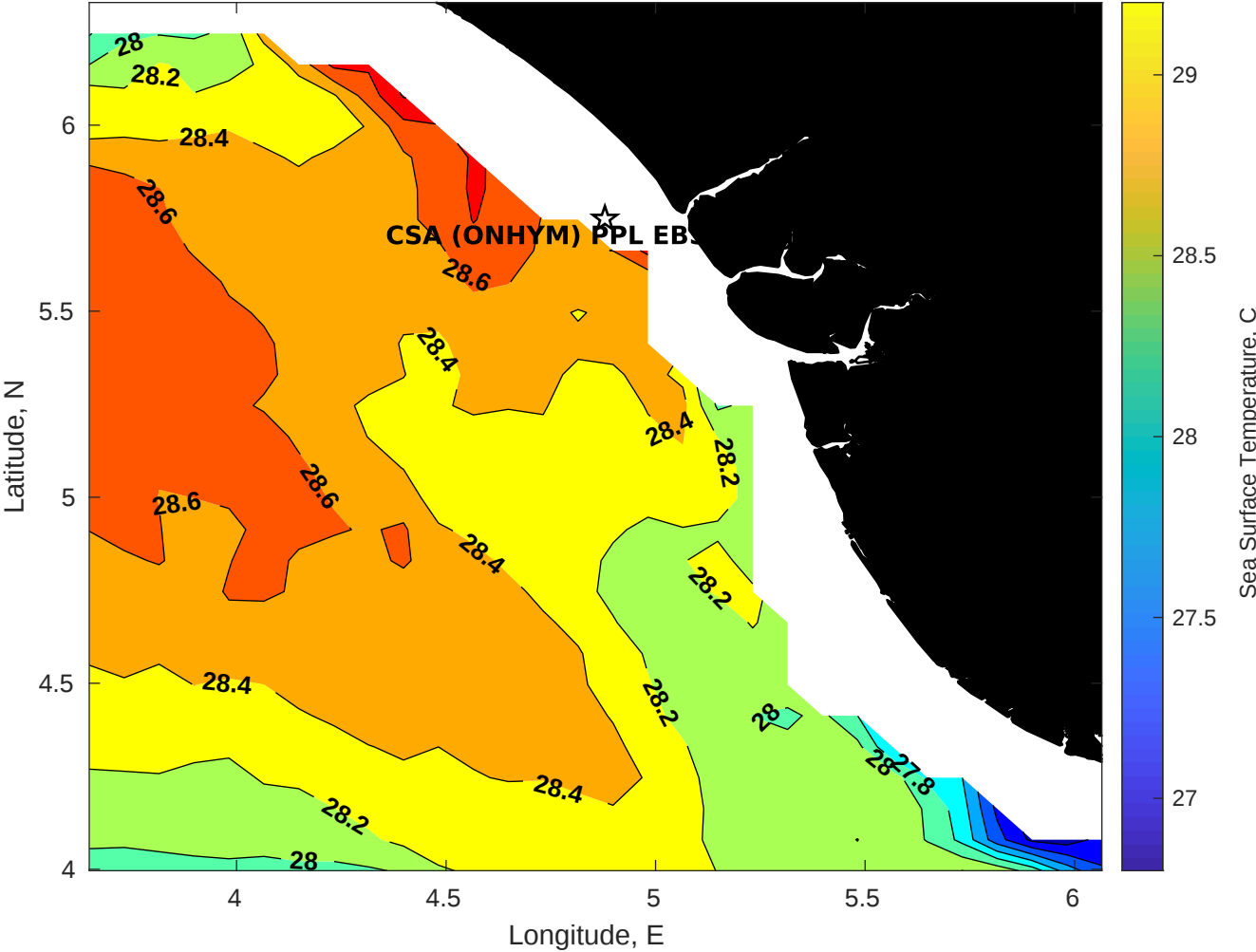
SST for CSA (ONHYM) PPL EBS - Nigeria at 05-Nov-2025 00:00:00
