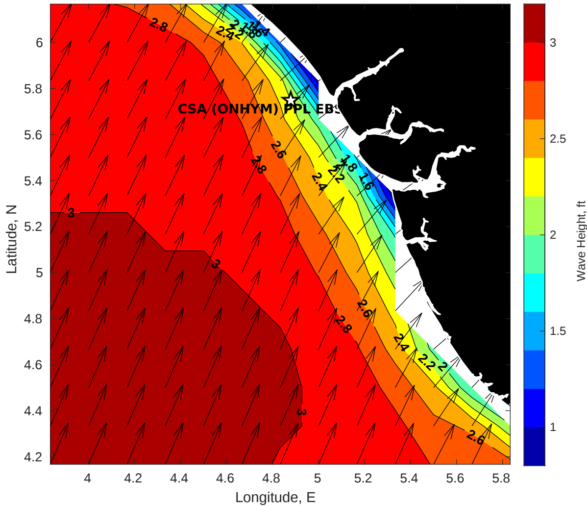
Wave Height (ft) for CSA (ONHYM) PPL EBS - Nigeria at 06-Nov-2025 09:00:00
