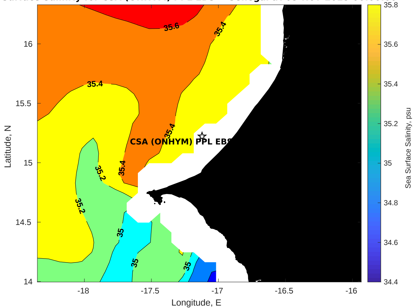
Surface Salinity for CSA (ONHYM) PPL EBS - Senegal at 05-Nov-2025 00:00:00
