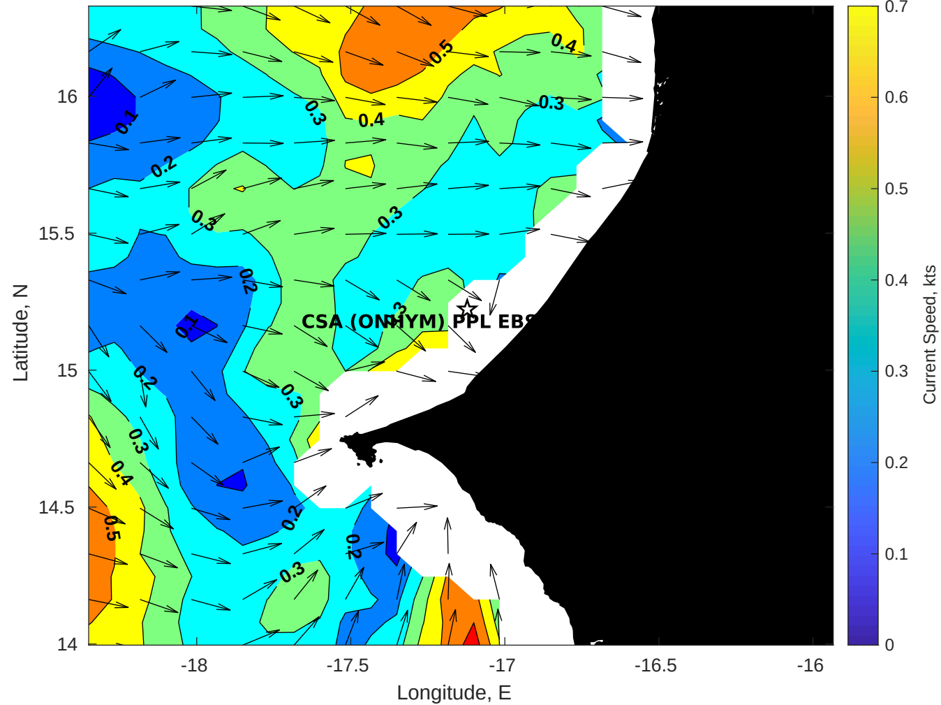
Surface Currents for CSA (ONHYM) PPL EBS - Senegal at 05-Nov-2025 00:00:00
