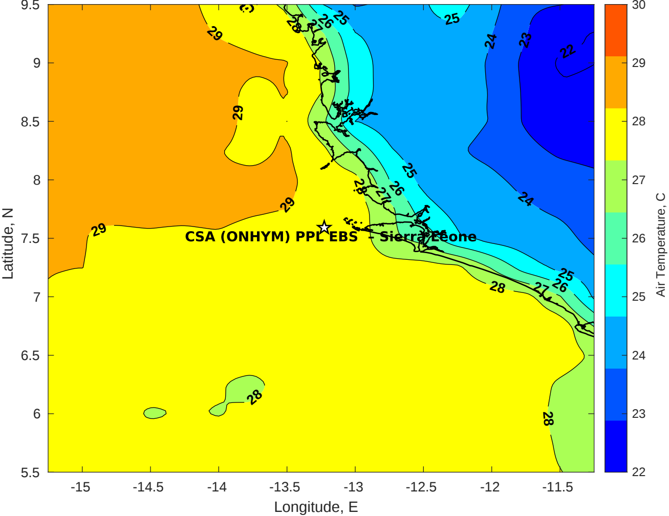
Air Temperature (C) for CSA (ONHYM) PPL EBS - Sierra Leone at 06-Nov-2025
