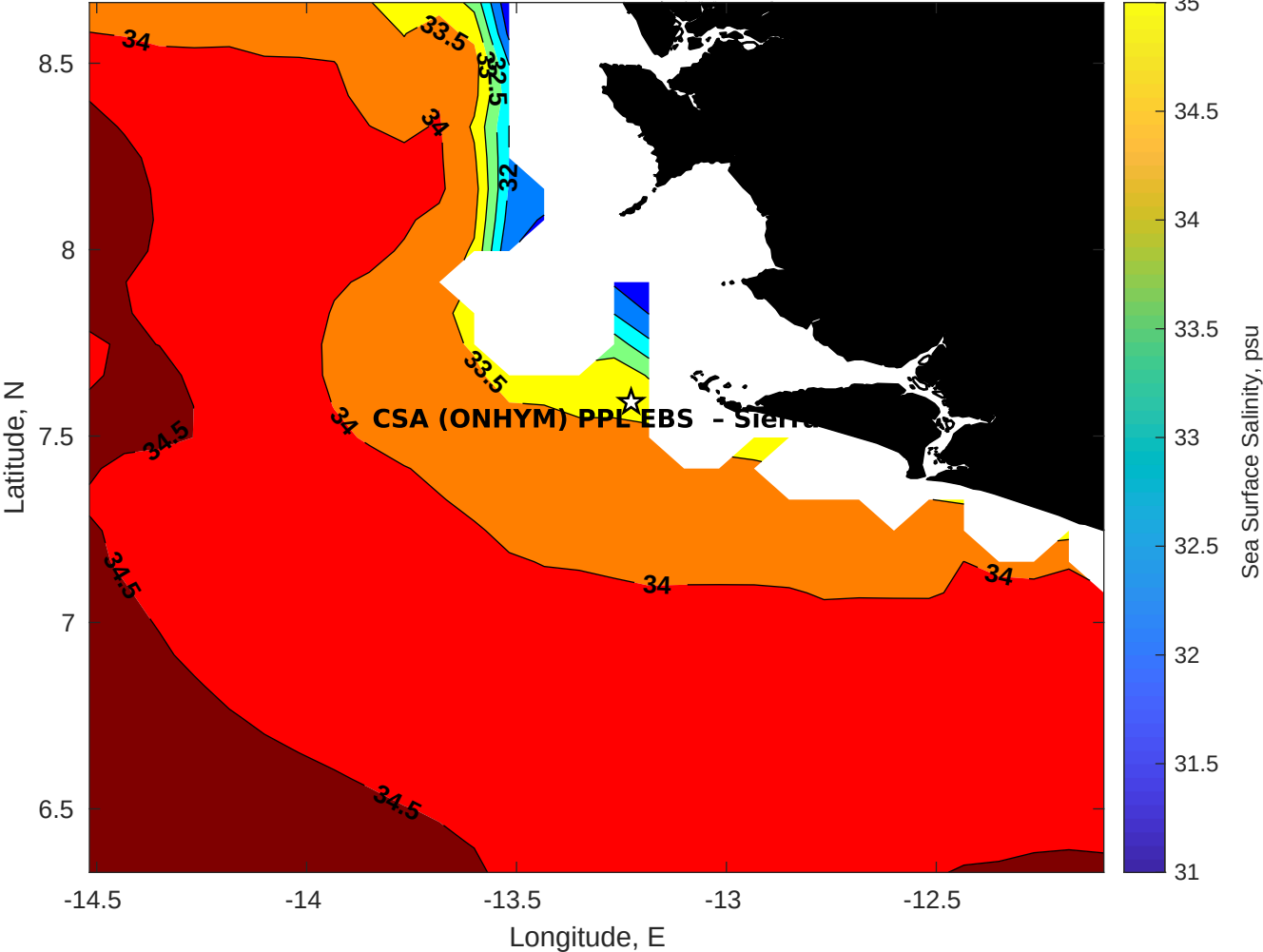
Surface Salinity for CSA (ONHYM) PPL EBS - Sierra Leone at 05-Nov-2025 00:00:00
