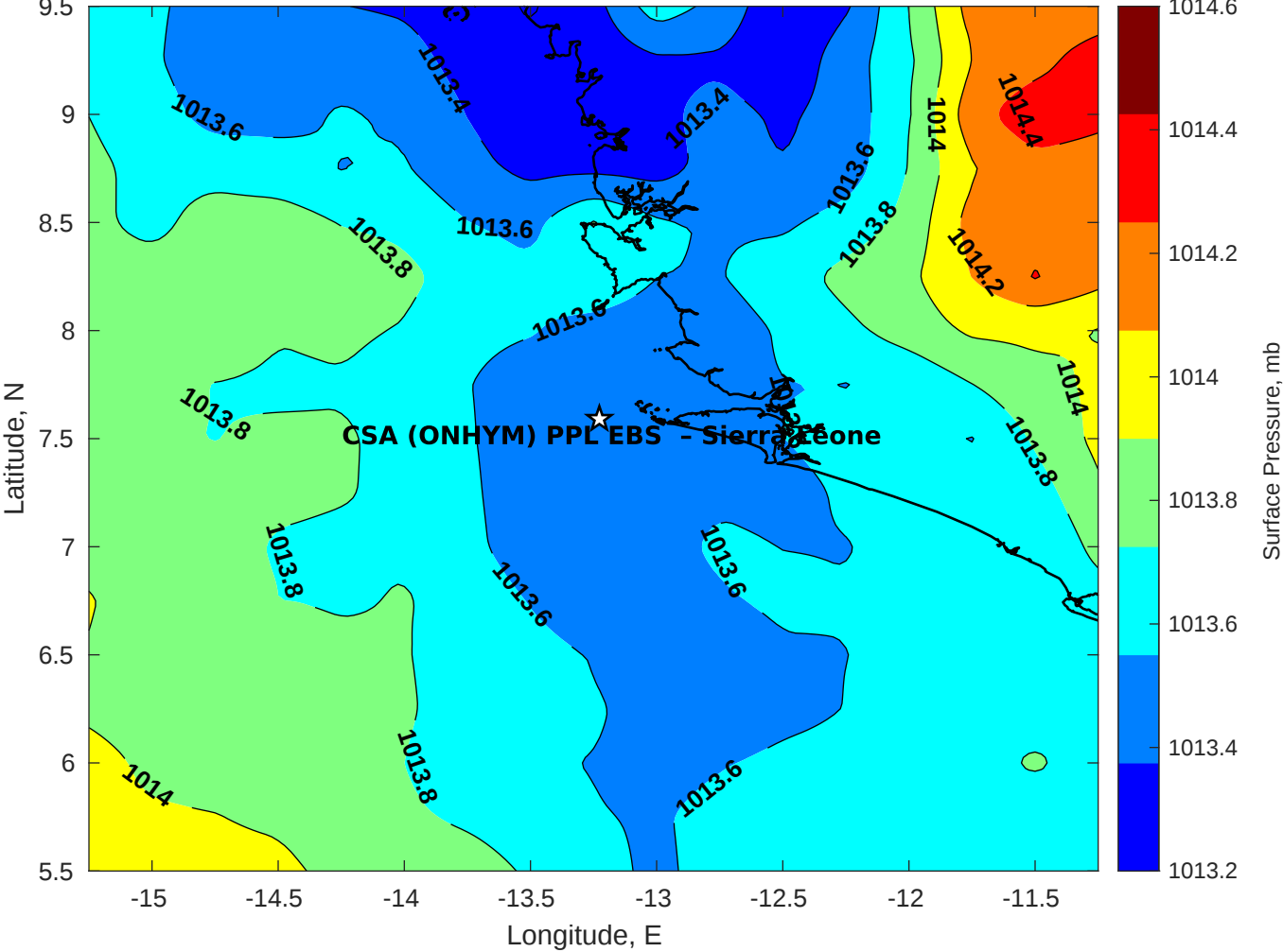
Surface Pressure (mb) for CSA (ONHYM) PPL EBS - Sierra Leone at 06-Nov-2025 00:00:00
