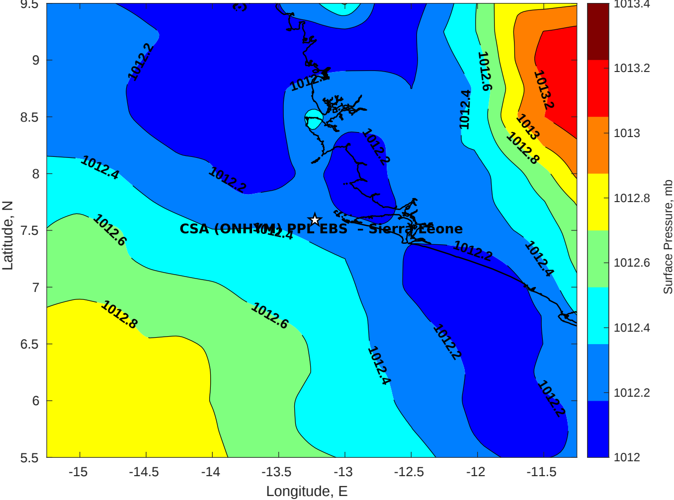
Surface Pressure (mb) for CSA (ONHYM) PPL EBS - Sierra Leone at 07-Nov-2025 00:00:00
