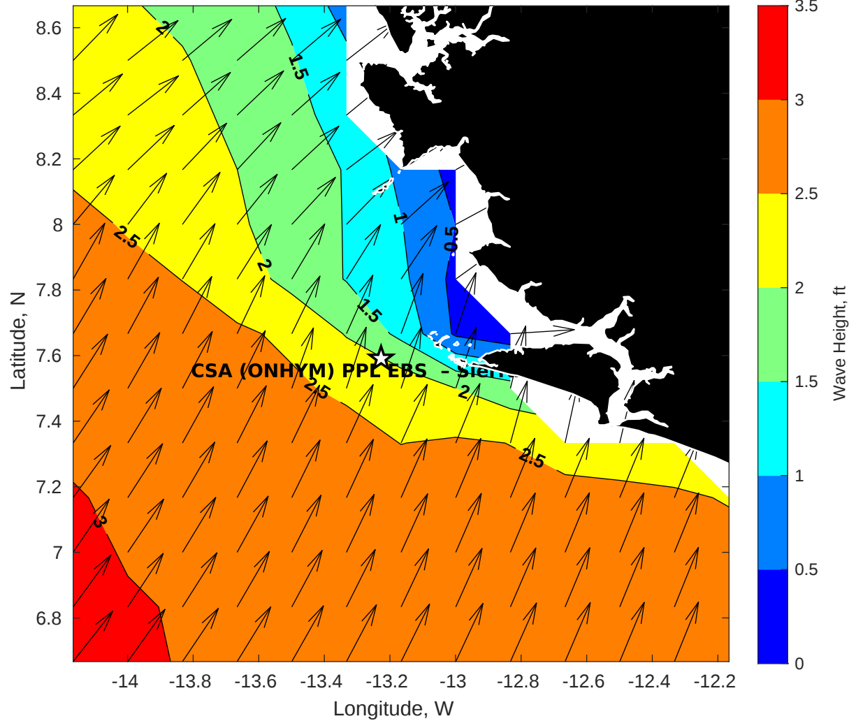
Wave Height (ft) for CSA (ONHYM) PPL EBS - Sierra Leone at 06-Nov-2025 09:00:00
