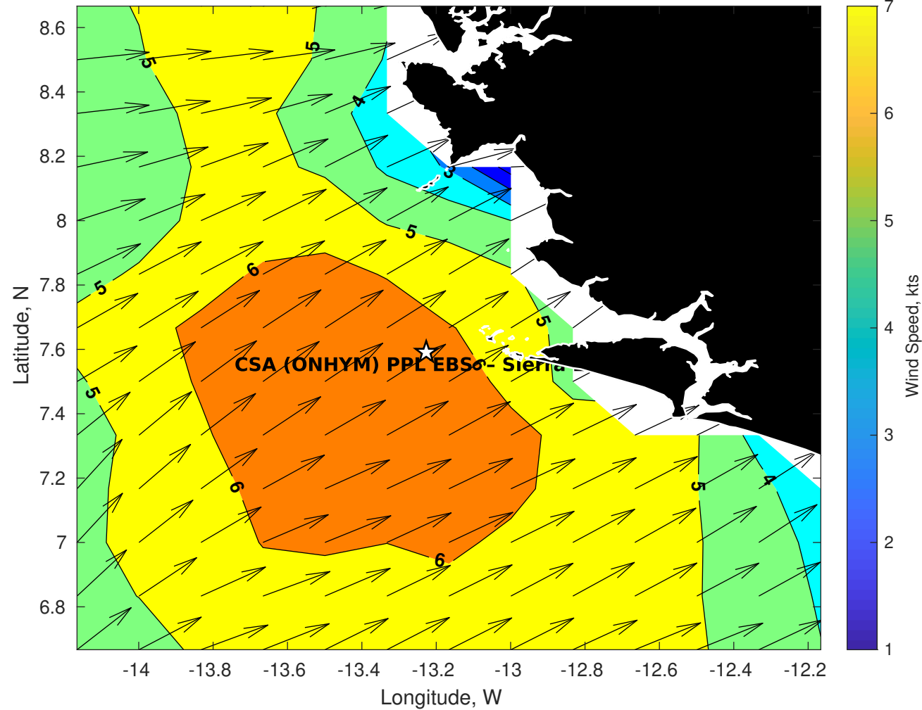
Winds (kts) for CSA (ONHYM) PPL EBS - Sierra Leone at 06-Nov-2025 09:00:00
