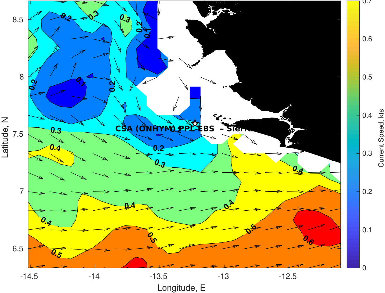
Surface Currents for CSA (ONHYM) PPL EBS - Sierra Leone at 05-Nov-2025 00:00:00
