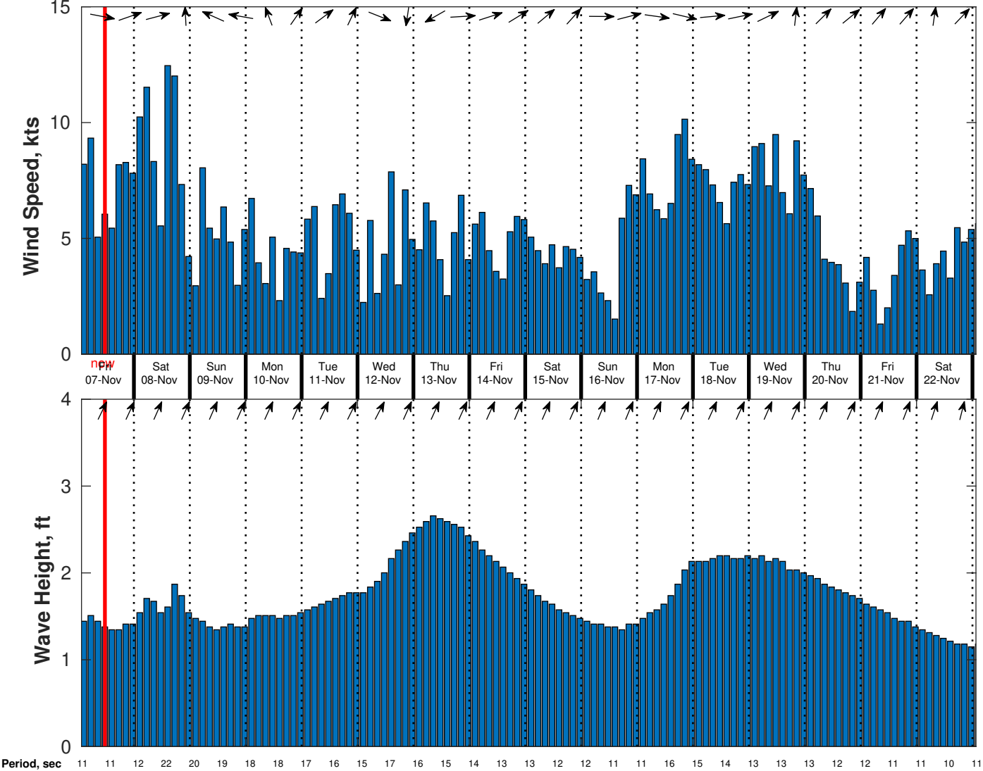
Wind & Wave Forecast for CSA (ONHYM) PPL EBS - Sierra Leone from 06-Nov-2025 01:00:00 to 22-Nov-2025 01:00:00
