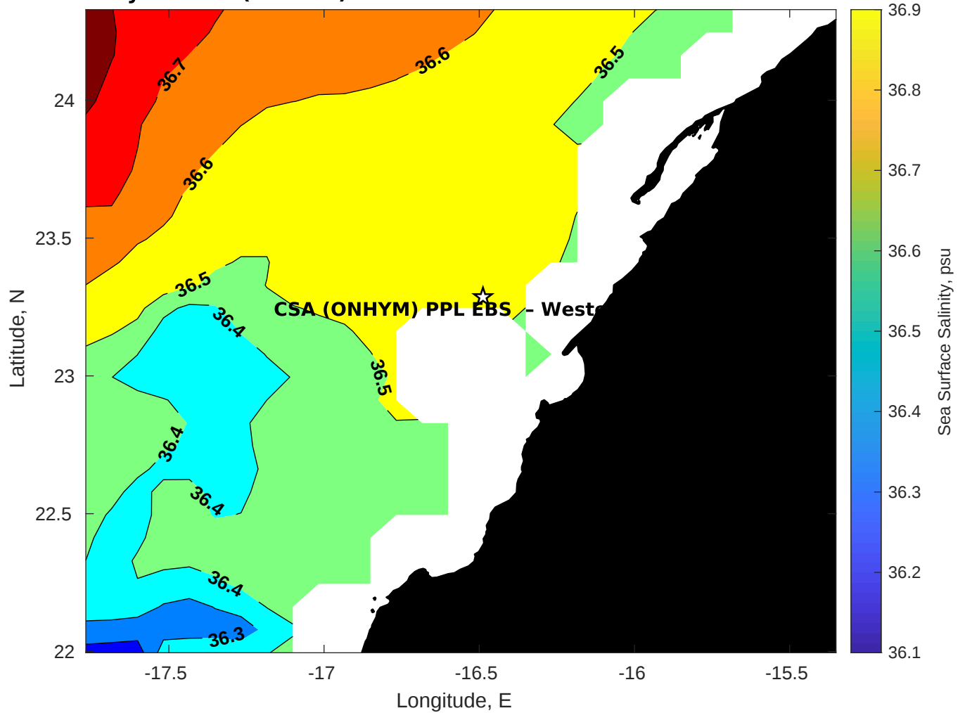
Surface Salinity for CSA (ONHYM) PPL EBS - Western Sahara at 05-Nov-2025 00:00:00
