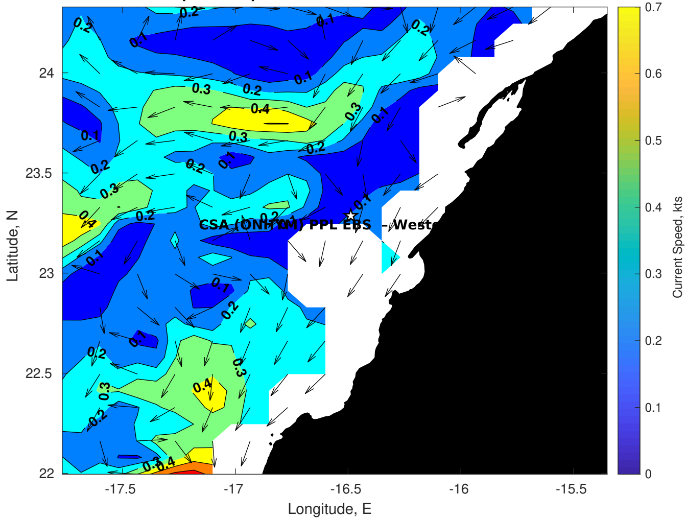
Surface Currents for CSA (ONHYM) PPL EBS - Western Sahara at 05-Nov-2025 00:00:00
