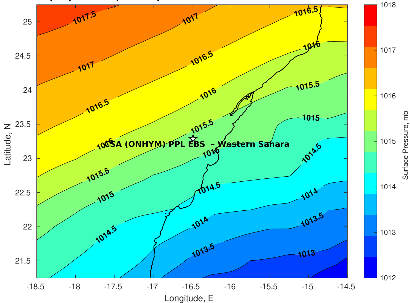
Surface Pressure (mb) for CSA (ONHYM) PPL EBS - Western Sahara at 07-Nov-2025 00:00:00
