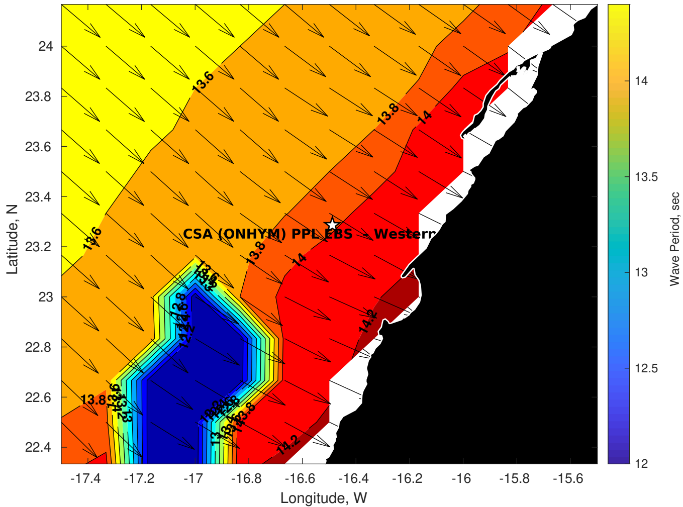
Wave Period (sec) for CSA (ONHYM) PPL EBS - Western Sahara at 06-Nov-2025 09:00:00
