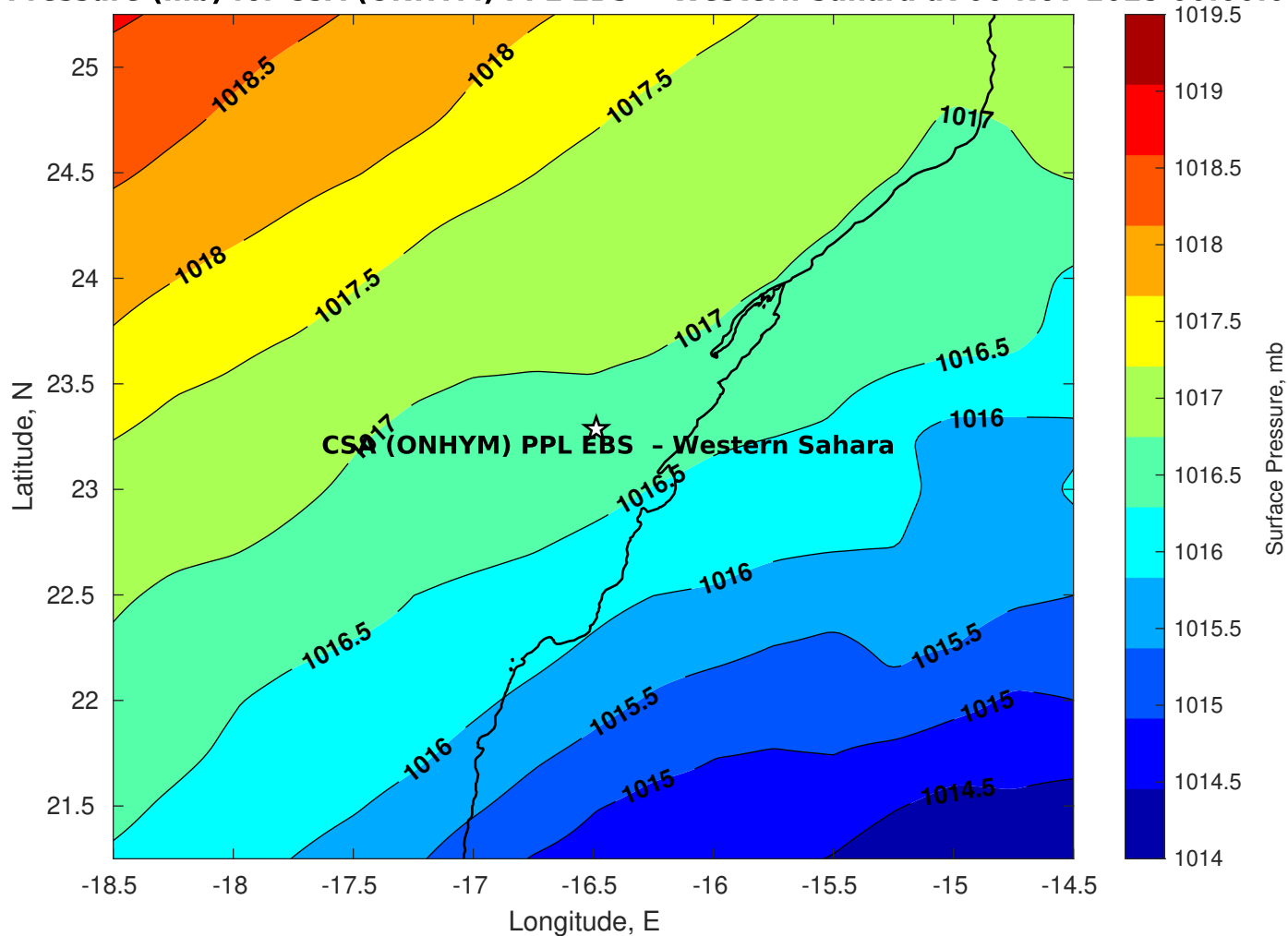
Surface Pressure (mb) for CSA (ONHYM) PPL EBS - Western Sahara at 06-Nov-2025 00:00:00
