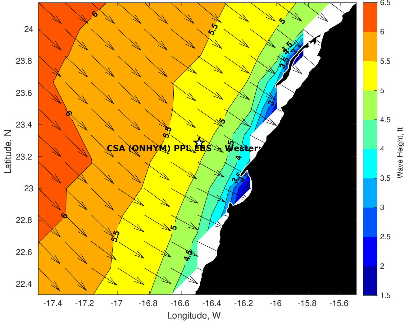
Wave Height (ft) for CSA (ONHYM) PPL EBS - Western Sahara at 06-Nov-2025 09:00:00
