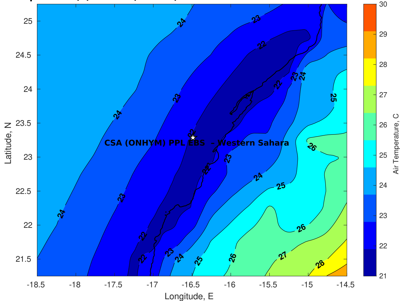
Air Temperature (C) for CSA (ONHYM) PPL EBS - Western Sahara at 06-Nov-2025
