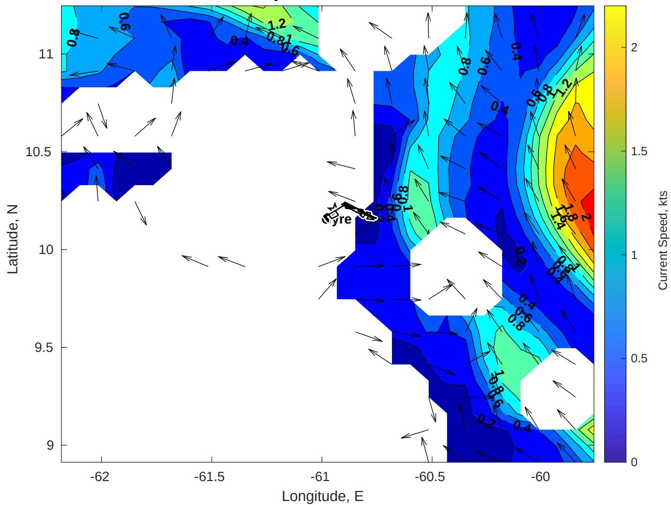
Surface Currents for Gyre at 05-Nov-2025 00:00:00
