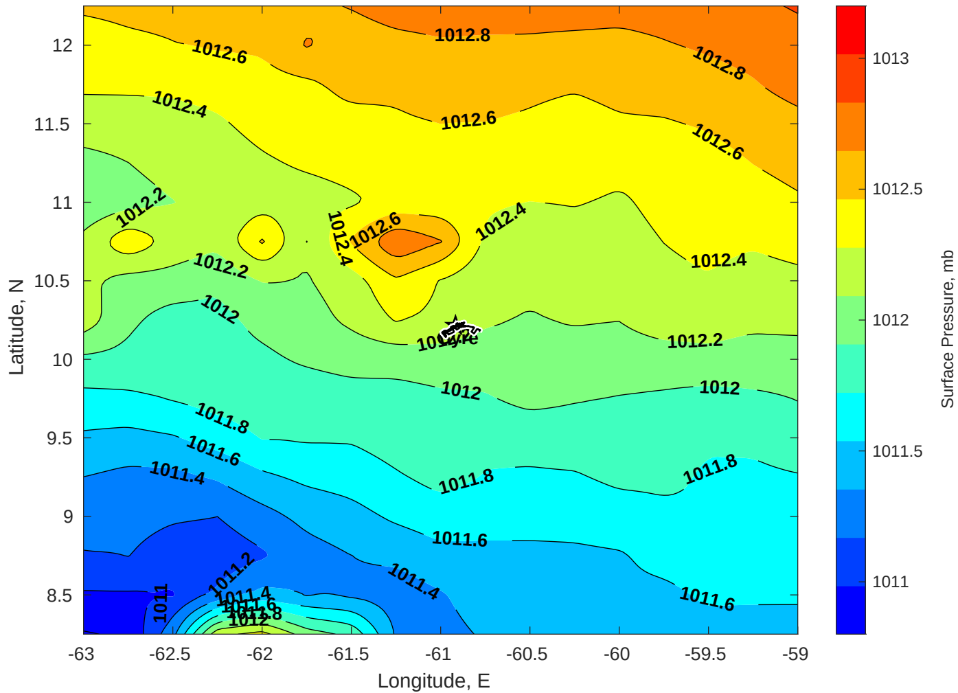
Surface Pressure (mb) for Gyre at 07-Nov-2025 00:00:00
