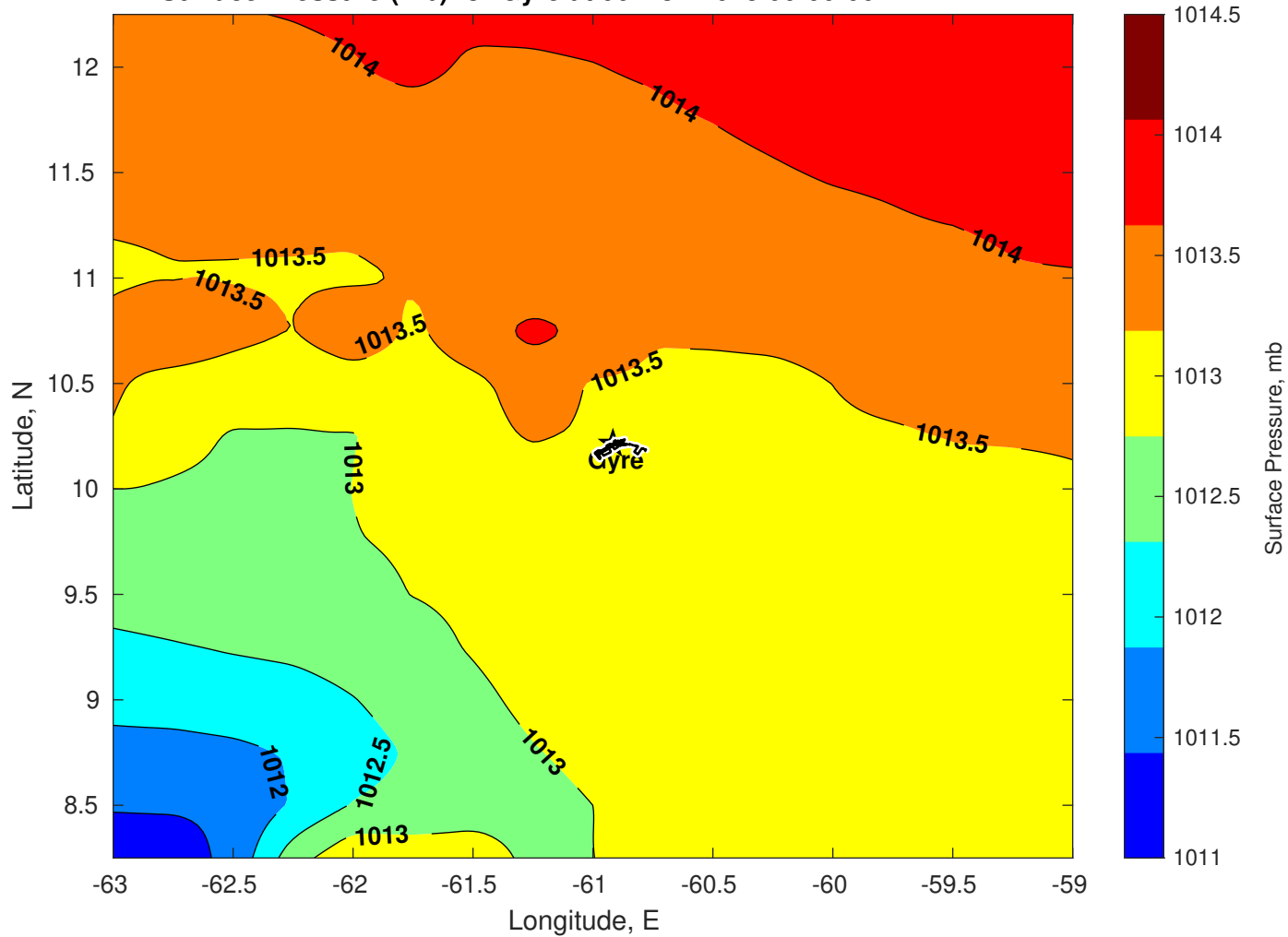
Surface Pressure (mb) for Gyre at 06-Nov-2025 00:00:00
