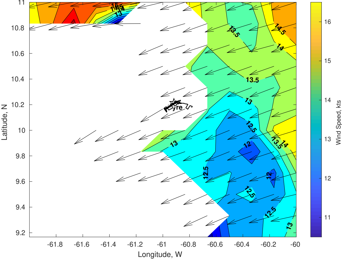
Winds (kts) for Gyre at 06-Nov-2025 09:00:00
