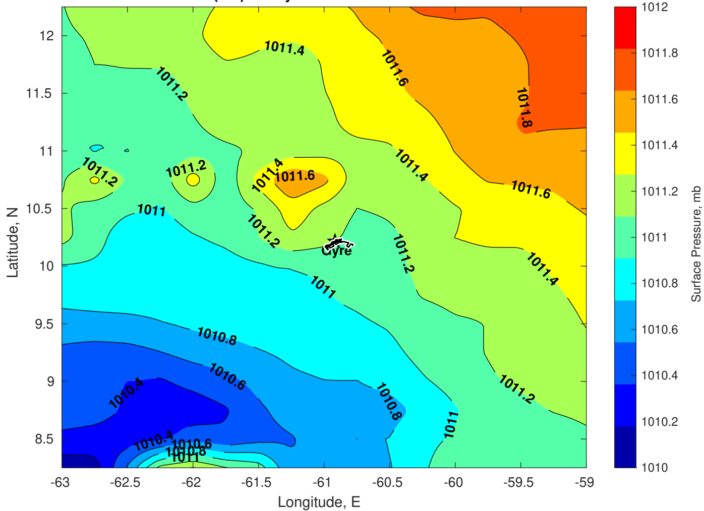
Surface Pressure (mb) for Gyre at 08-Nov-2025 00:00:00
