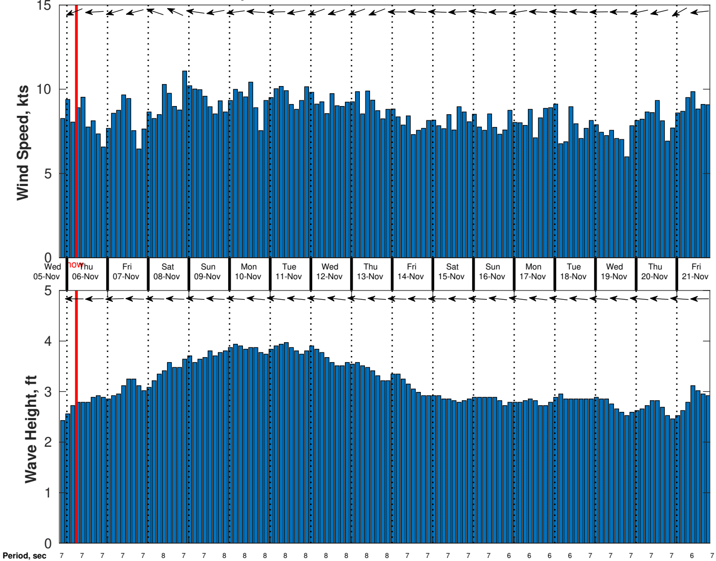
Wind & Wave Forecast for Gyre from 05-Nov-2025 20:00:00 to 21-Nov-2025 20:00:00
