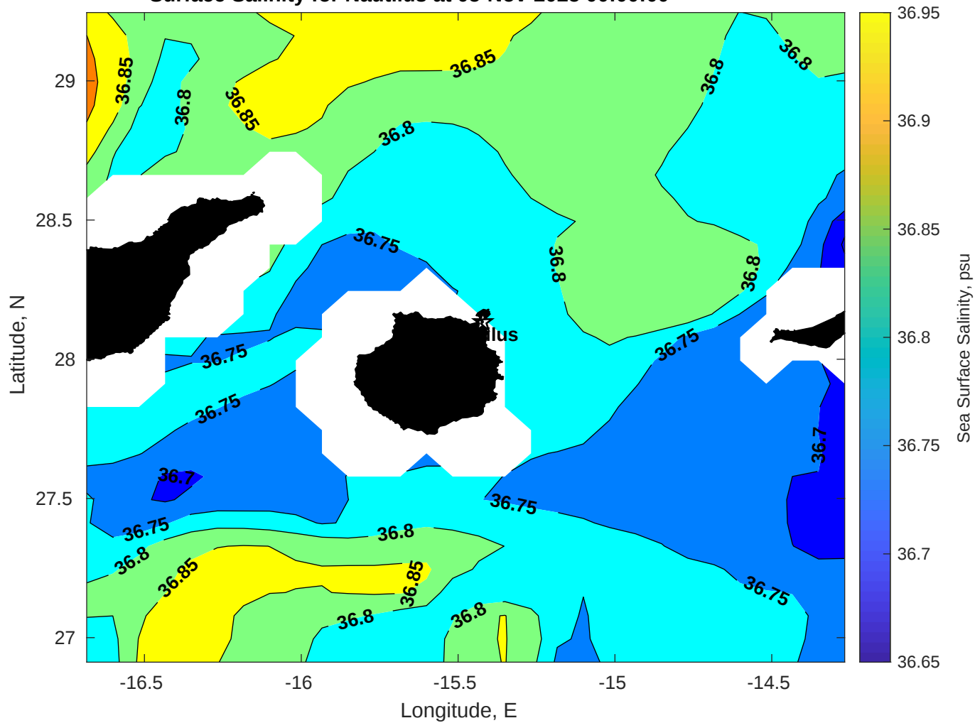
Surface Salinity for Nautilus at 05-Nov-2025 00:00:00
