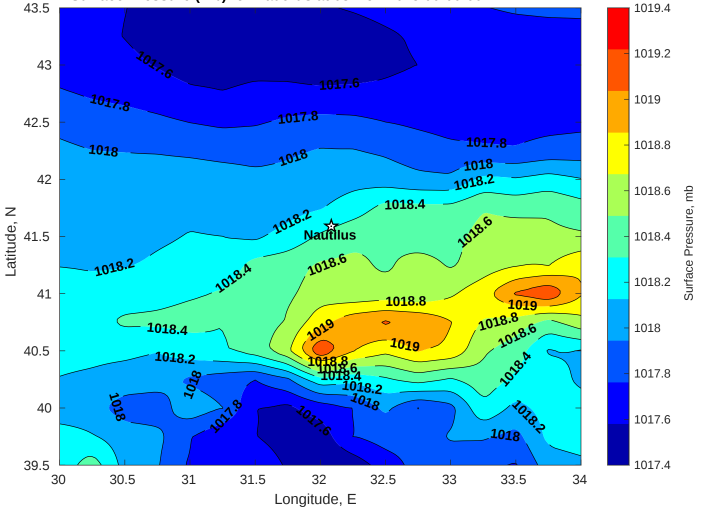
Surface Pressure (mb) for Nautilus at 08-Nov-2025 00:00:00
