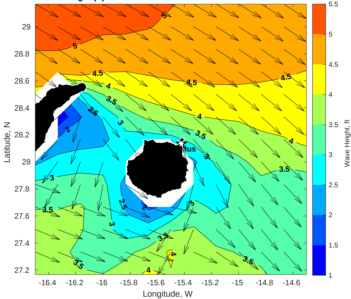
Wave Height (ft) for Nautilus at 05-Nov-2025 21:00:00
