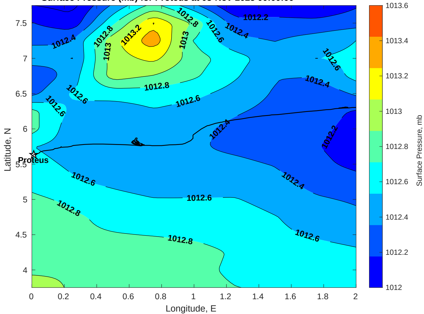
Surface Pressure (mb) for Proteus at 08-Nov-2025 00:00:00
