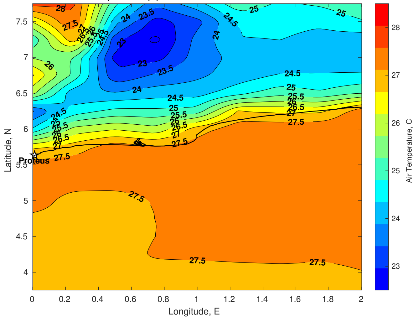
Air Temperature (C) for Proteus at 06-Nov-2025
