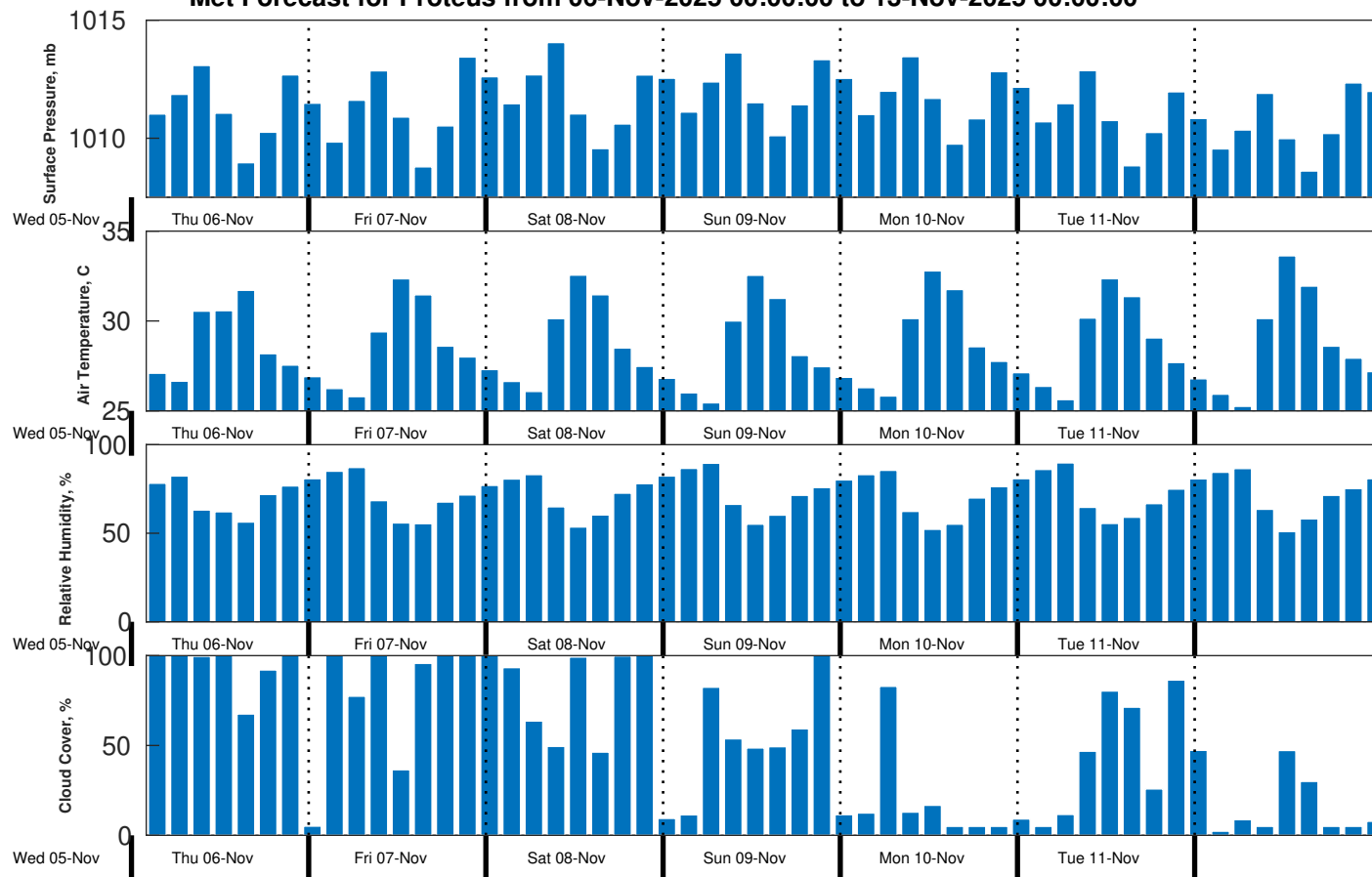
Met Forecast for Proteus from 06-Nov-2025 00:00:00 to 13-Nov-2025 00:00:00
