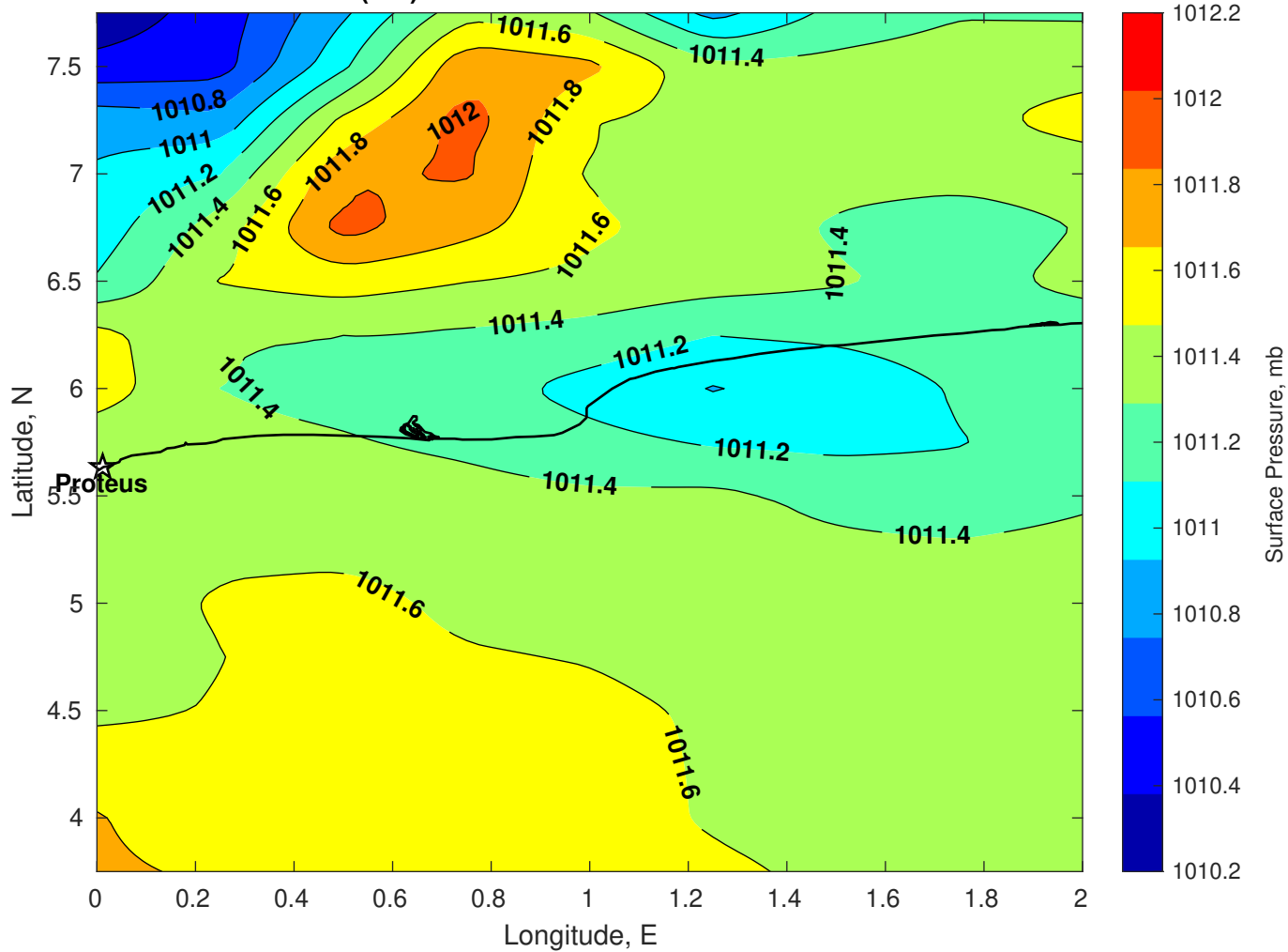
Surface Pressure (mb) for Proteus at 07-Nov-2025 00:00:00
