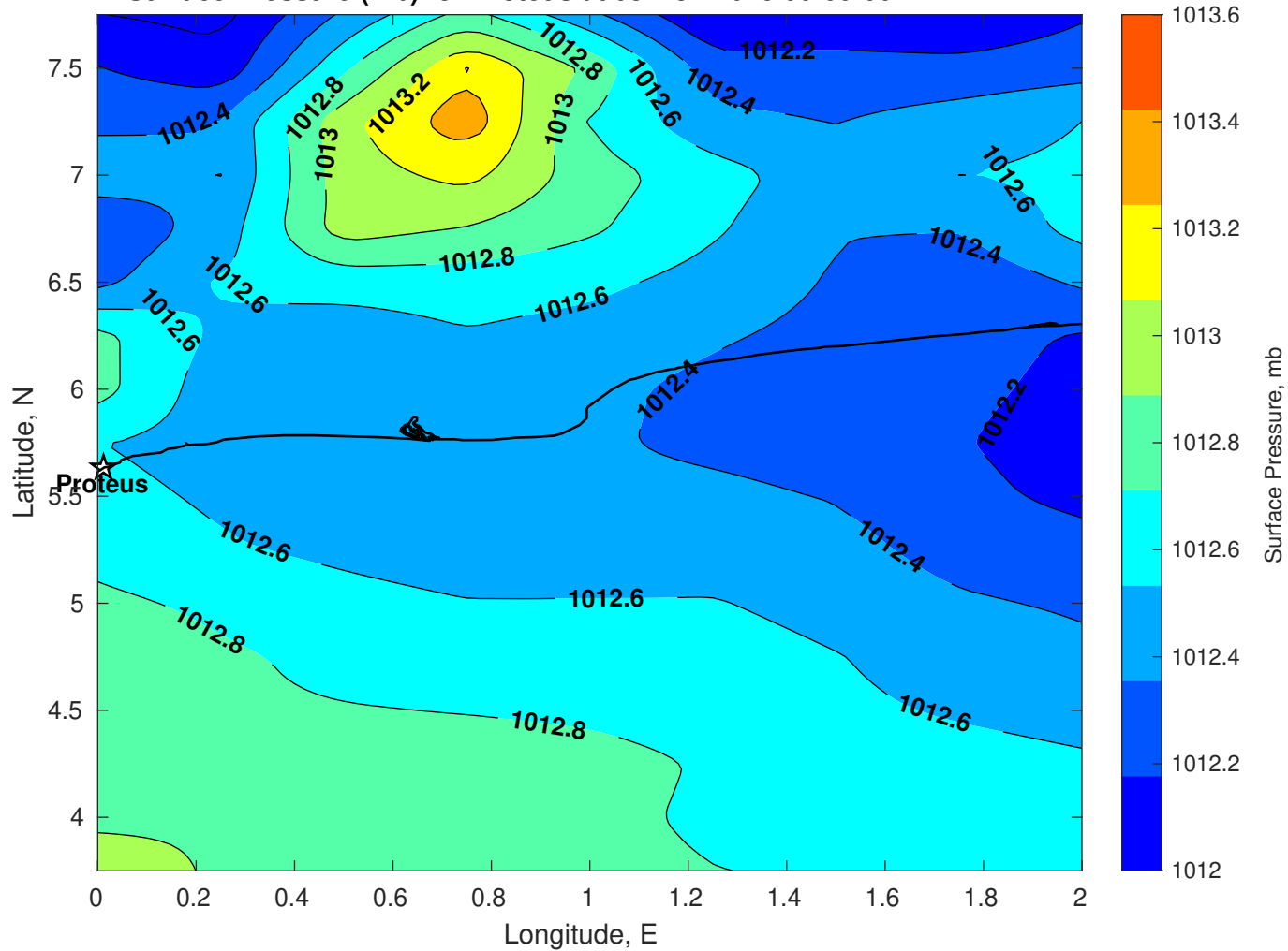
Surface Pressure (mb) for Proteus at 08-Nov-2025 00:00:00
