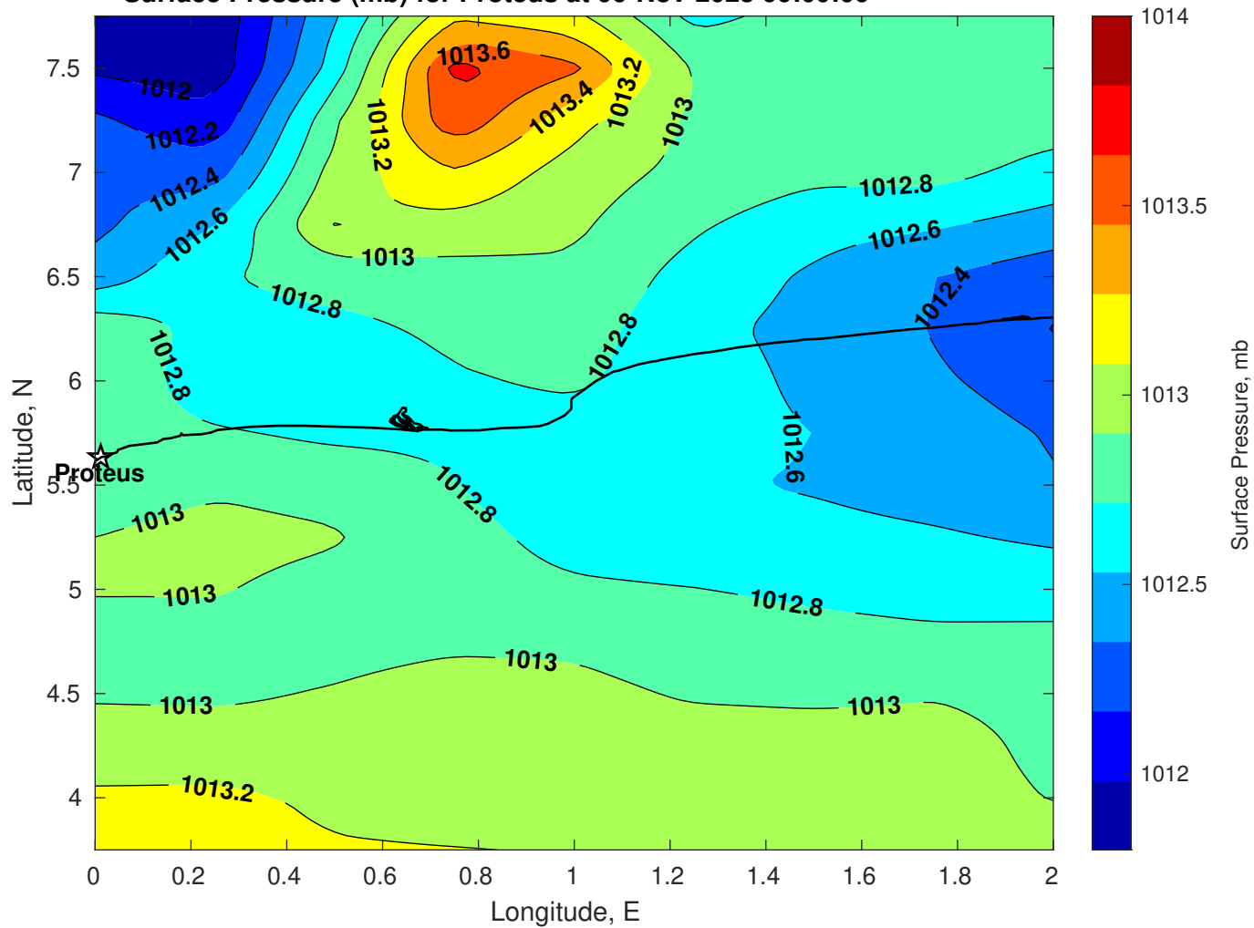
Surface Pressure (mb) for Proteus at 06-Nov-2025 00:00:00
