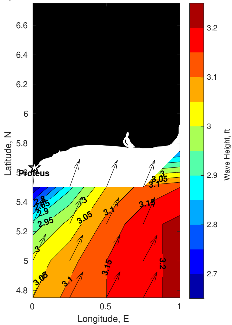
Wave Height (ft) for Proteus at 06-Nov-2025 09:00:00
