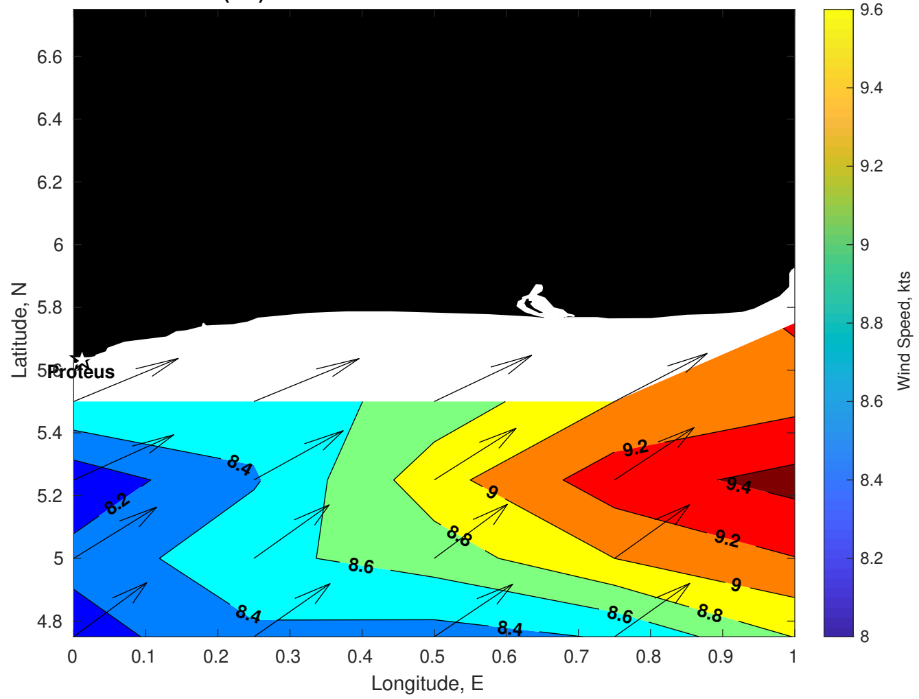
Winds (kts) for Proteus at 06-Nov-2025 09:00:00
