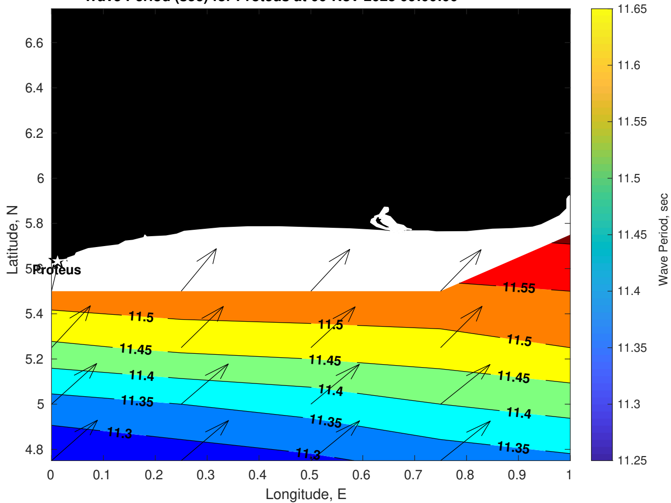
Wave Period (sec) for Proteus at 06-Nov-2025 09:00:00
