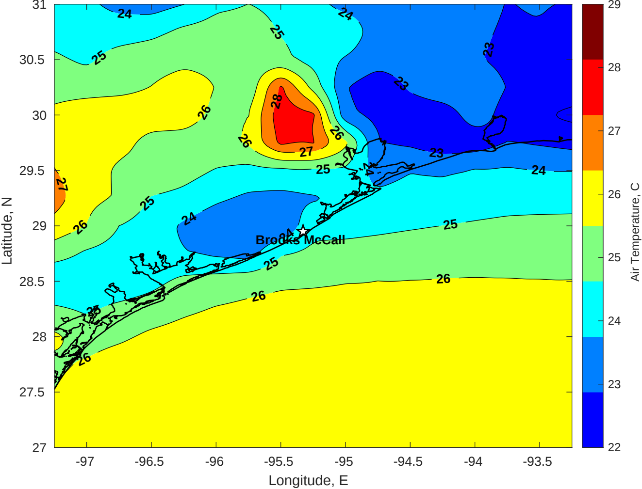
Air Temperature (C) for Brooks McCall at 07-Nov-2025
