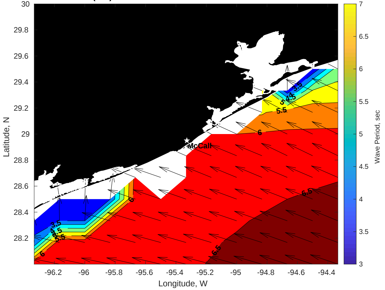
Wave Period (sec) for Brooks McCall at 07-Nov-2025 09:00:00
