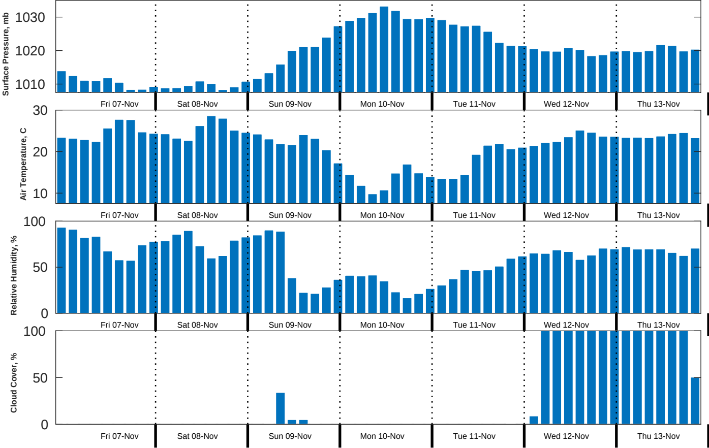
Met Forecast for Brooks McCall from 07-Nov-2025 00:00:00 to 14-Nov-2025 00:00:00
