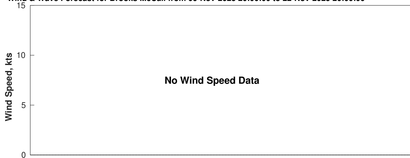
Wind & Wave Forecast for Brooks McCall from 06-Nov-2025 20:00:00 to 22-Nov-2025 20:00:00
