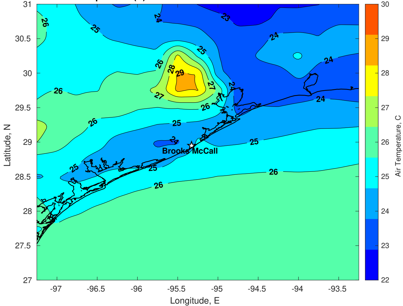
Air Temperature (C) for Brooks McCall at 07-Nov-2025
