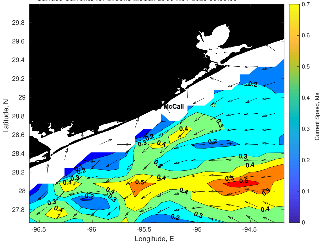
Surface Currents for Brooks McCall at 06-Nov-2025 00:00:00
