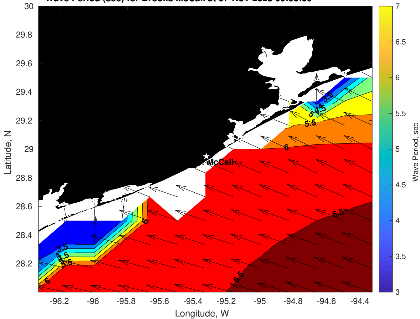
Wave Period (sec) for Brooks McCall at 07-Nov-2025 09:00:00
