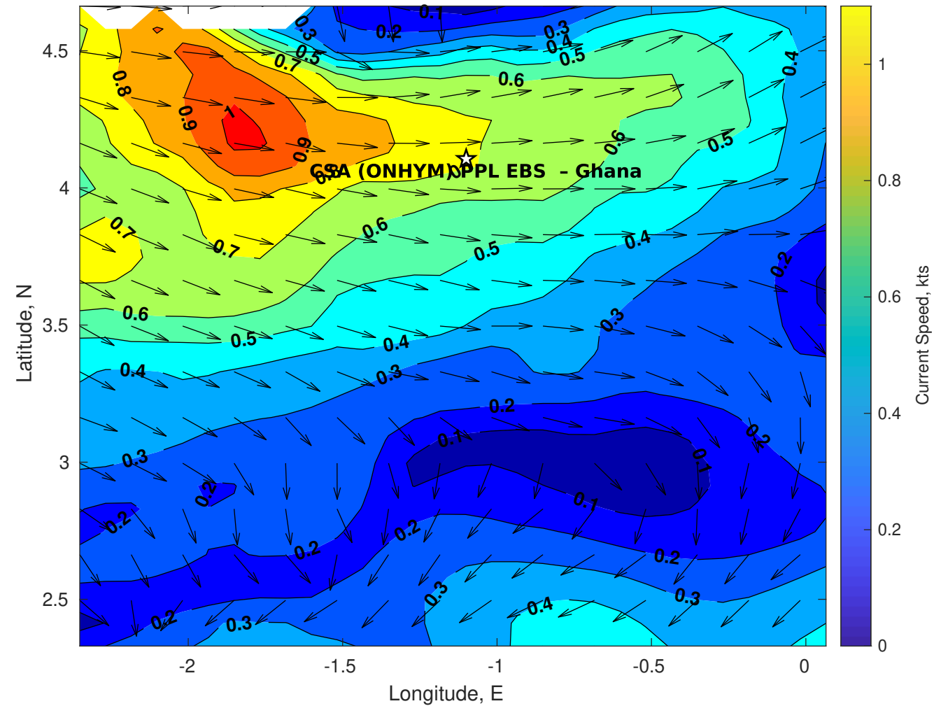
Surface Currents for CSA (ONHYM) PPL EBS - Ghana at 06-Nov-2025 00:00:00
