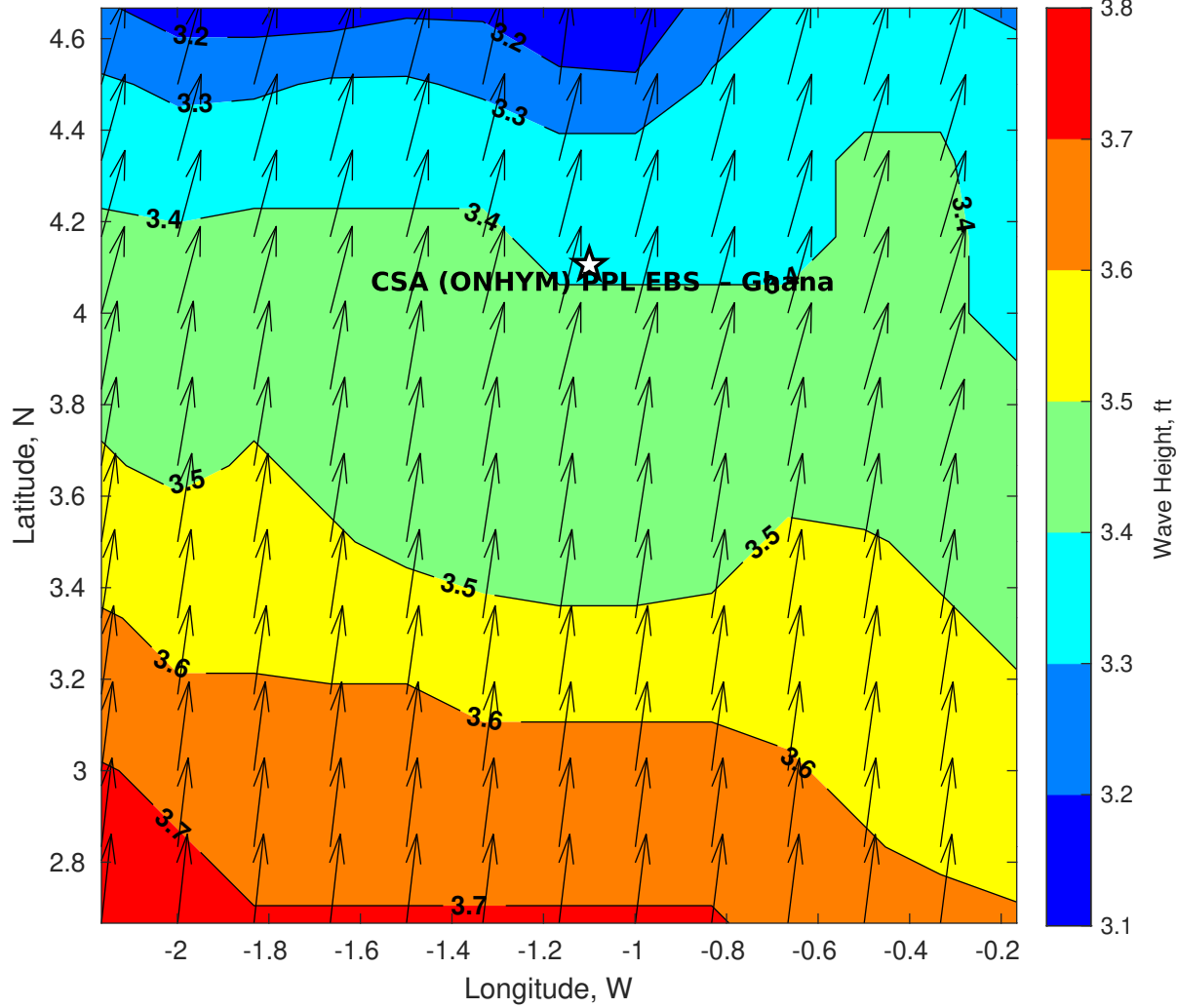
Wave Height (ft) for CSA (ONHYM) PPL EBS - Ghana at 07-Nov-2025 09:00:00
