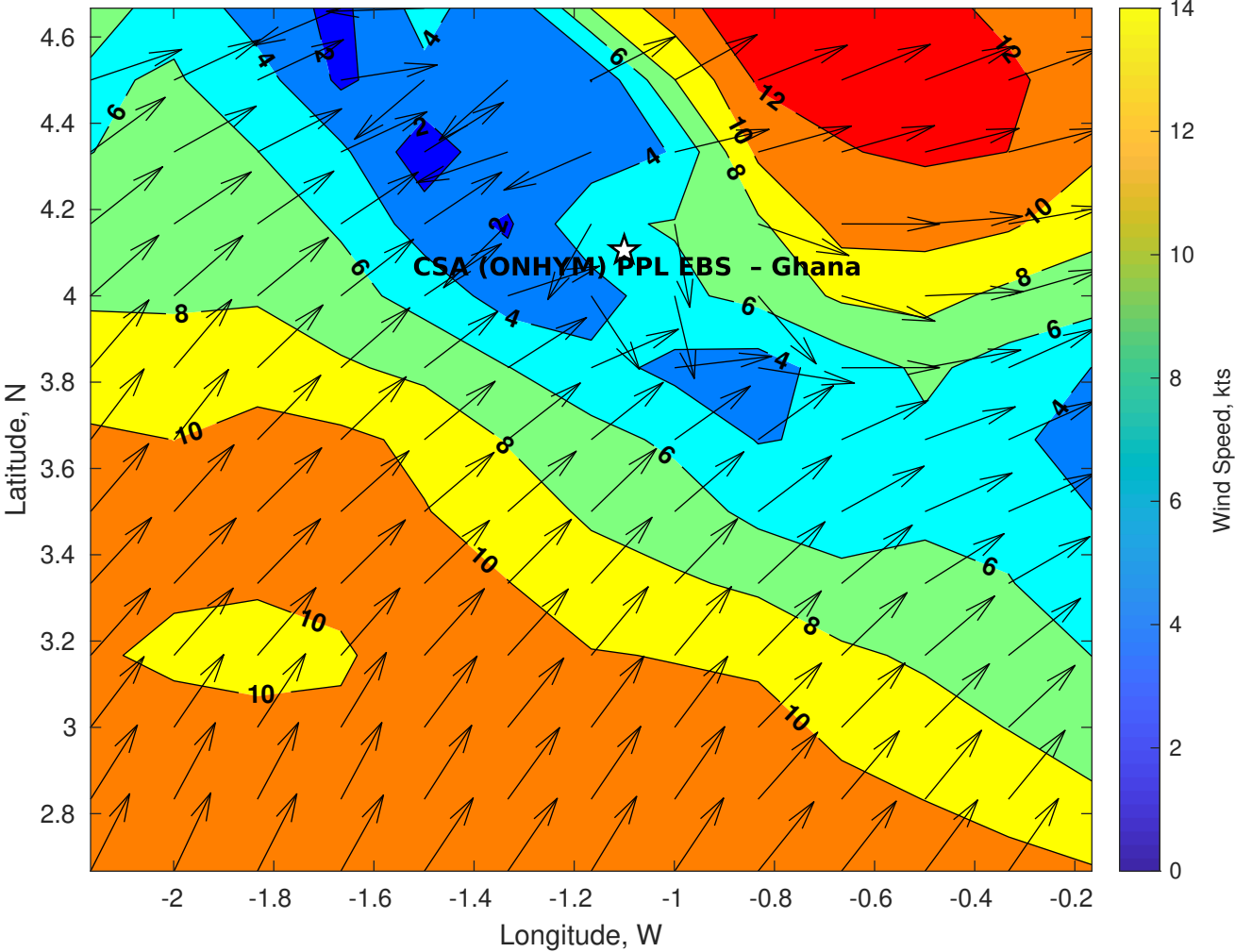
Winds (kts) for CSA (ONHYM) PPL EBS - Ghana at 07-Nov-2025 09:00:00
