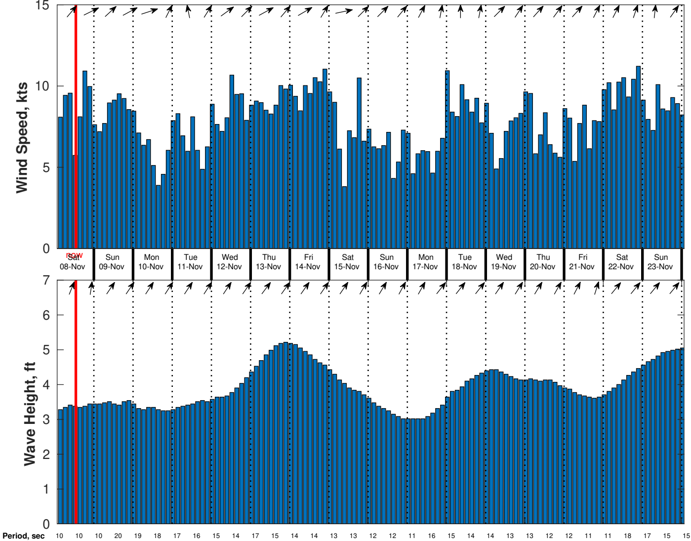
Wind & Wave Forecast for CSA (ONHYM) PPL EBS - Ghana from 07-Nov-2025 02:00:00 to 23-Nov-2025 02:00:00
