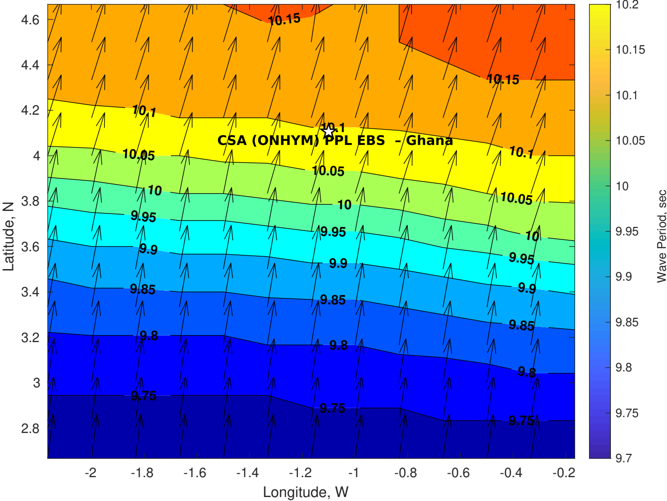
Wave Period (sec) for CSA (ONHYM) PPL EBS - Ghana at 07-Nov-2025 09:00:00
