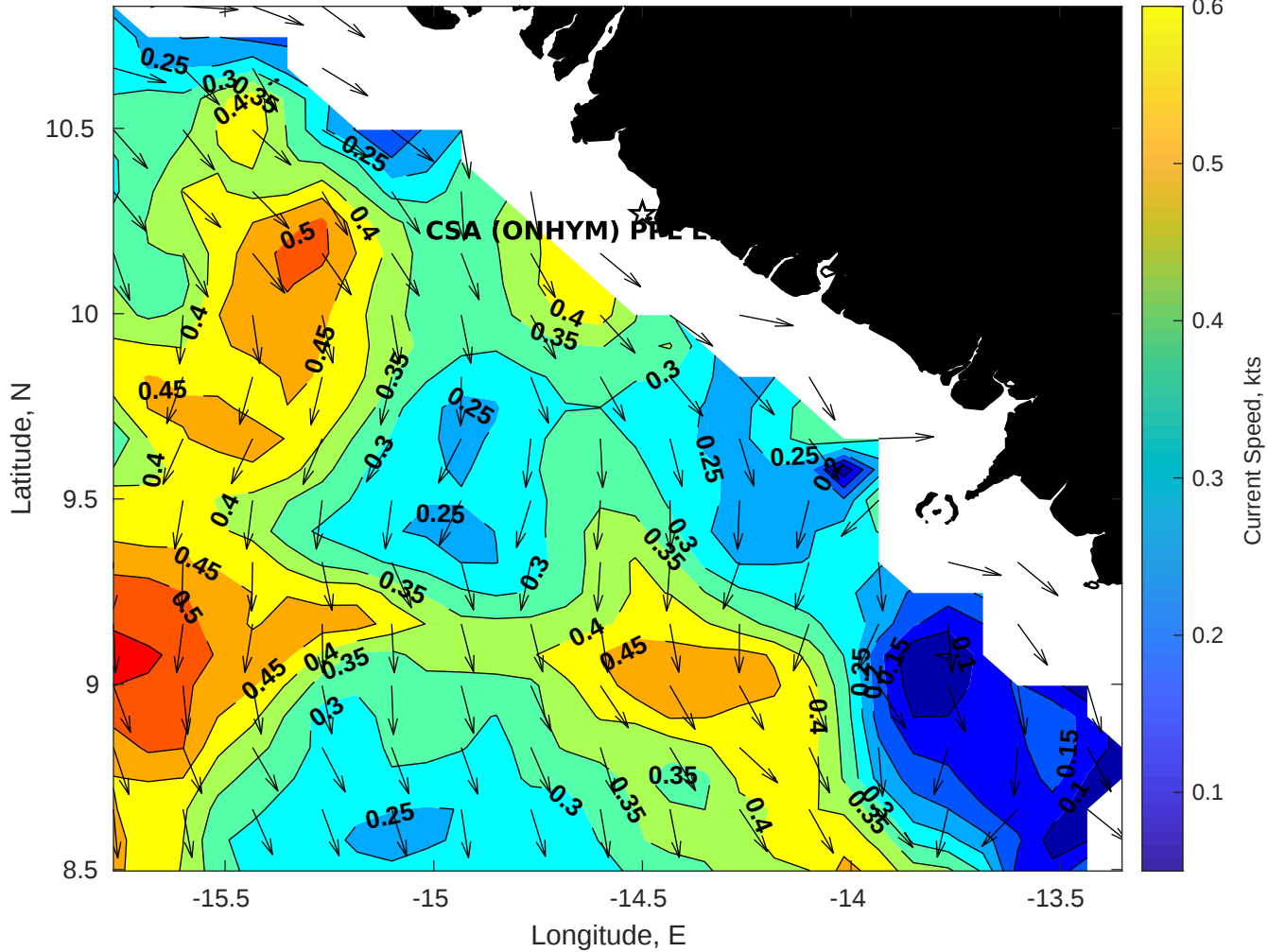
Surface Currents for CSA (ONHYM) PPL EBS - Guinea at 06-Nov-2025 00:00:00
