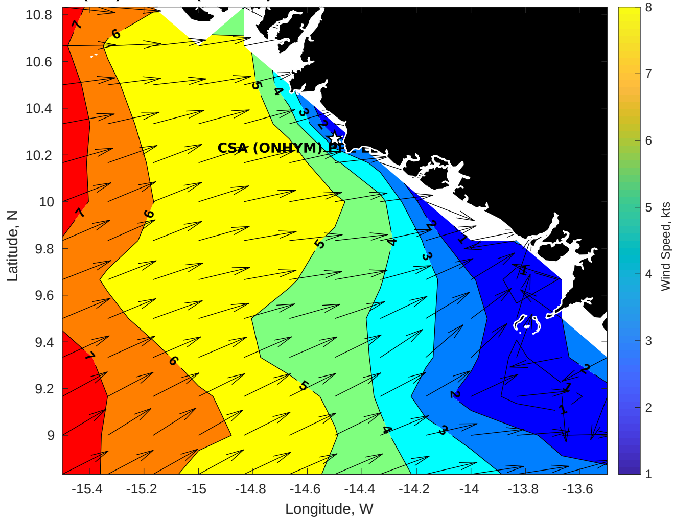
Winds (kts) for CSA (ONHYM) PPL EBS - Guinea at 07-Nov-2025 09:00:00
