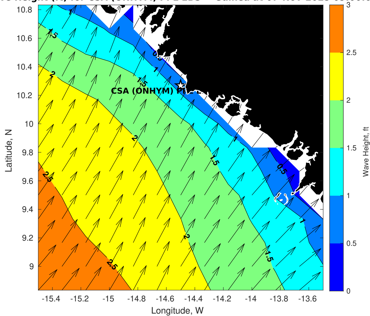
Wave Height (ft) for CSA (ONHYM) PPL EBS - Guinea at 07-Nov-2025 09:00:00
