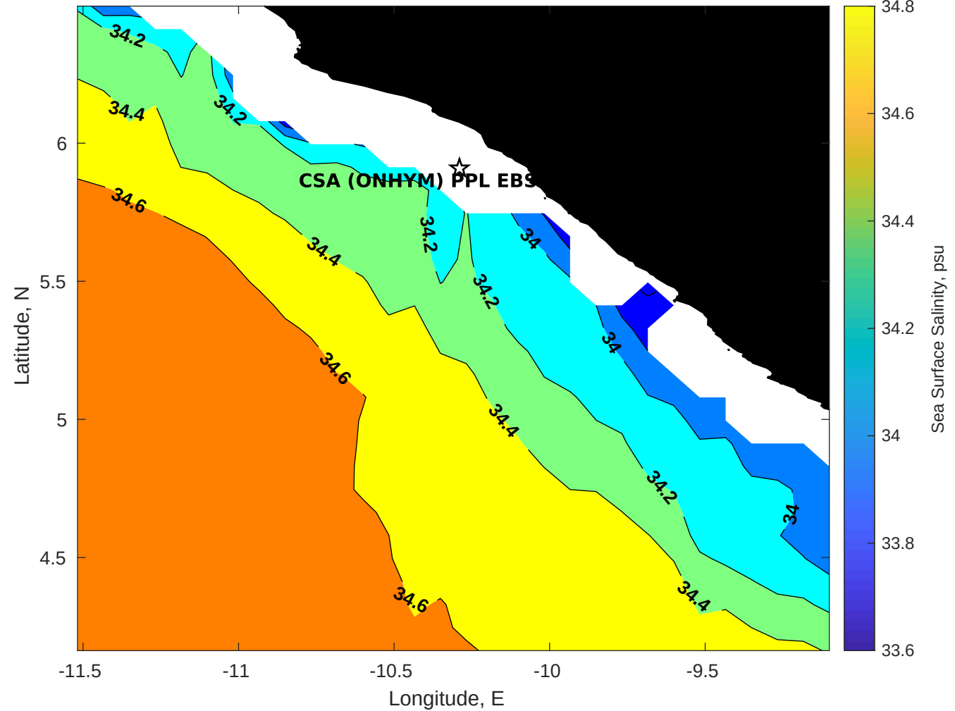
Surface Salinity for CSA (ONHYM) PPL EBS - Liberia at 06-Nov-2025 00:00:00
