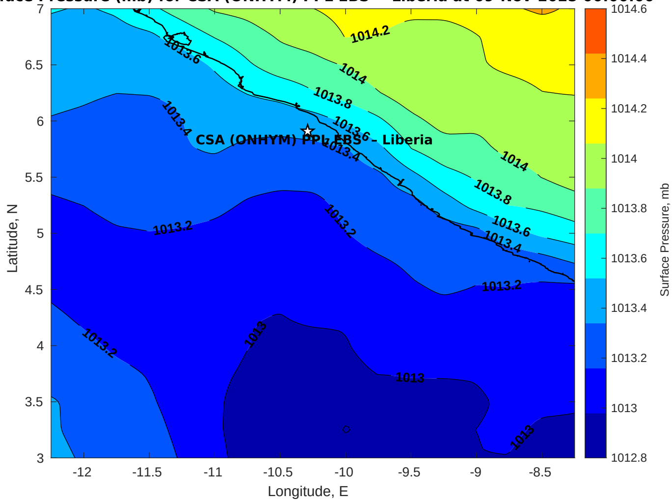
Surface Pressure (mb) for CSA (ONHYM) PPL EBS - Liberia at 09-Nov-2025 00:00:00
