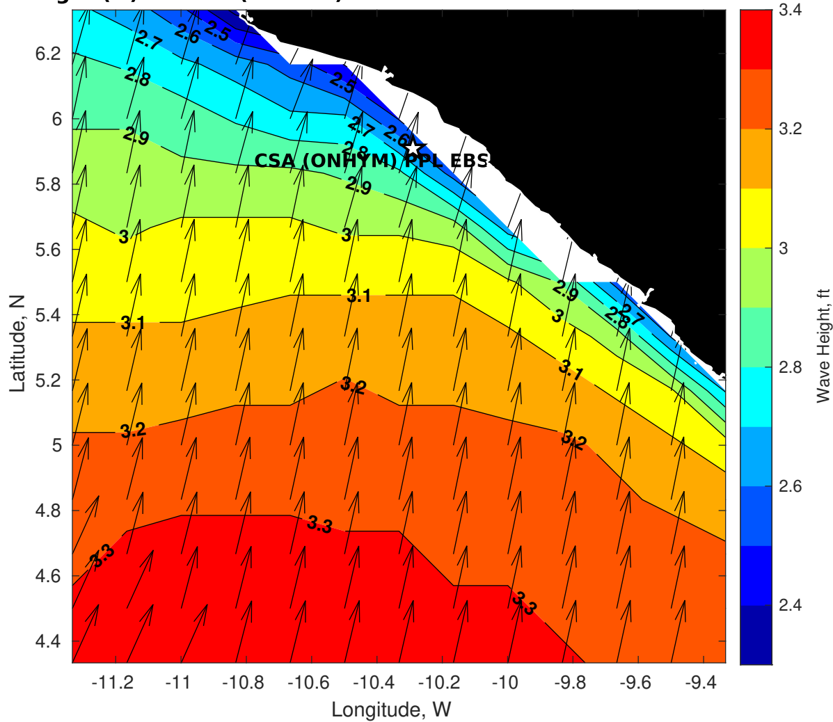
Wave Height (ft) for CSA (ONHYM) PPL EBS - Liberia at 07-Nov-2025 09:00:00
