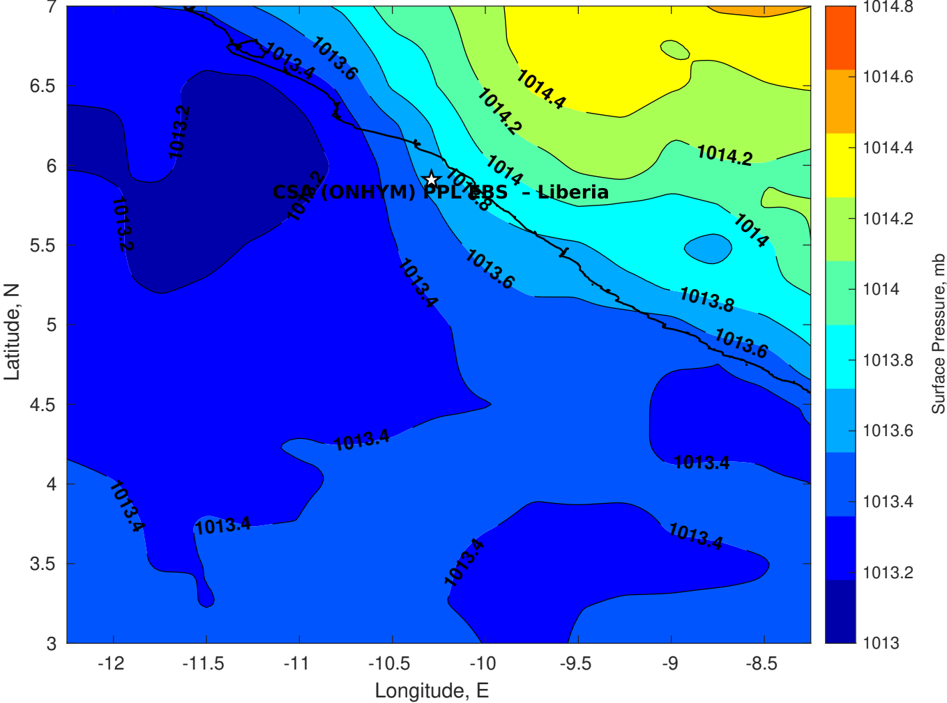
Surface Pressure (mb) for CSA (ONHYM) PPL EBS - Liberia at 08-Nov-2025 00:00:00
