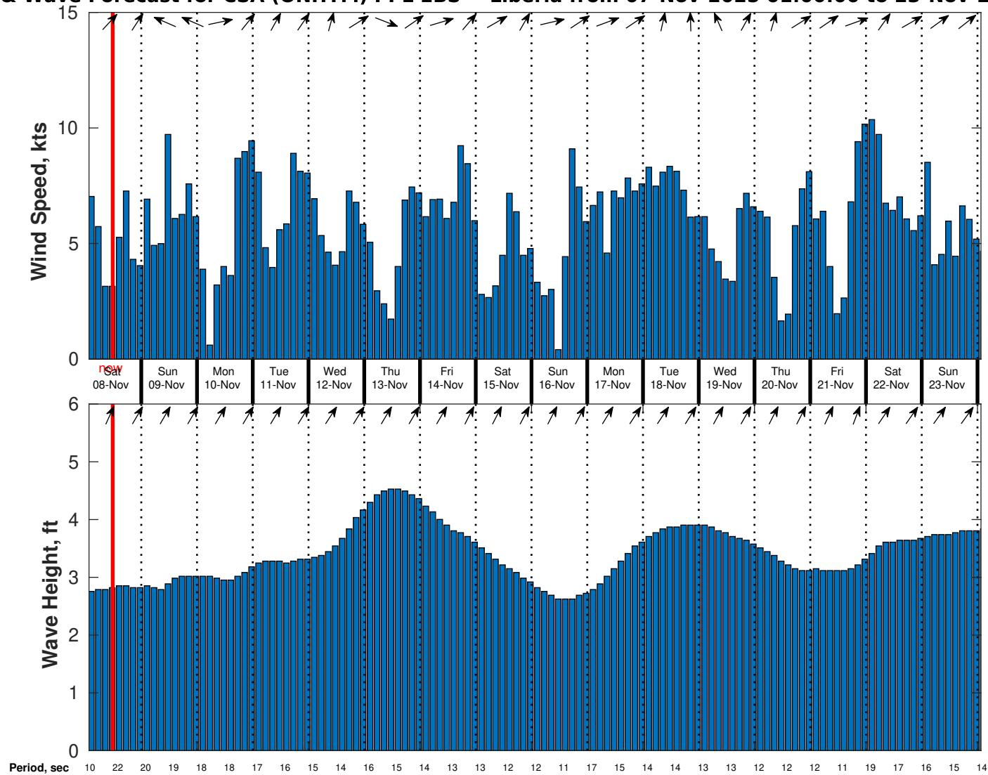
Wind & Wave Forecast for CSA (ONHYM) PPL EBS - Liberia from 07-Nov-2025 01:00:00 to 23-Nov-2025 01:00:00
