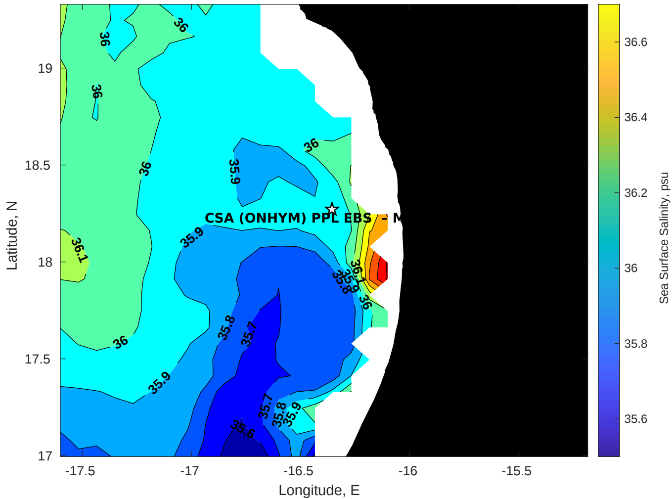
Surface Salinity for CSA (ONHYM) PPL EBS - Mauritania at 06-Nov-2025 00:00:00
