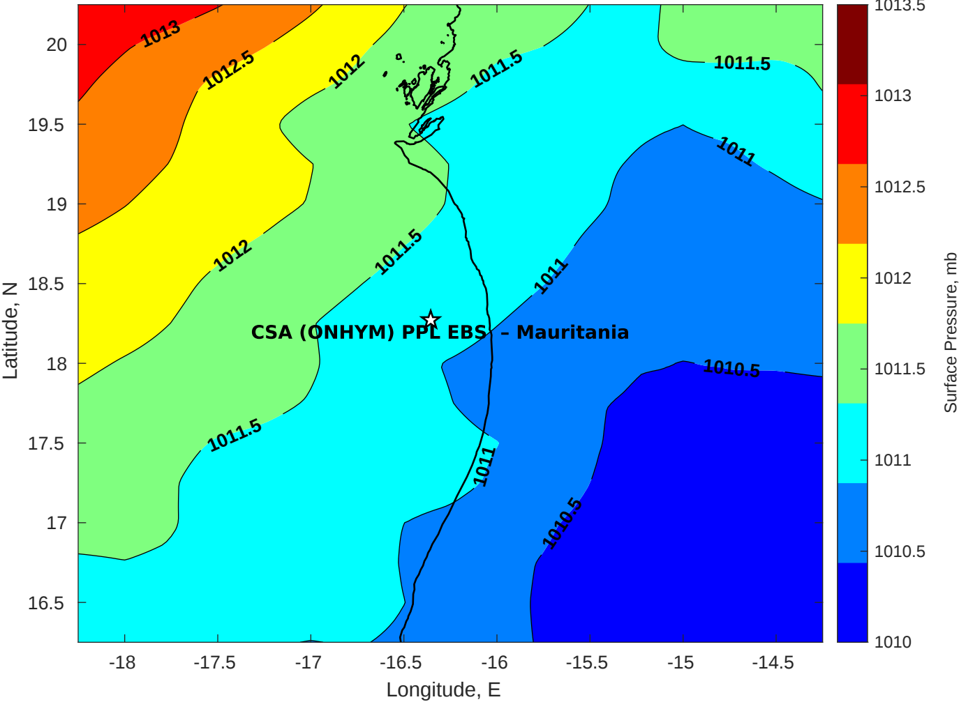
Surface Pressure (mb) for CSA (ONHYM) PPL EBS - Mauritania at 07-Nov-2025 00:00:00
