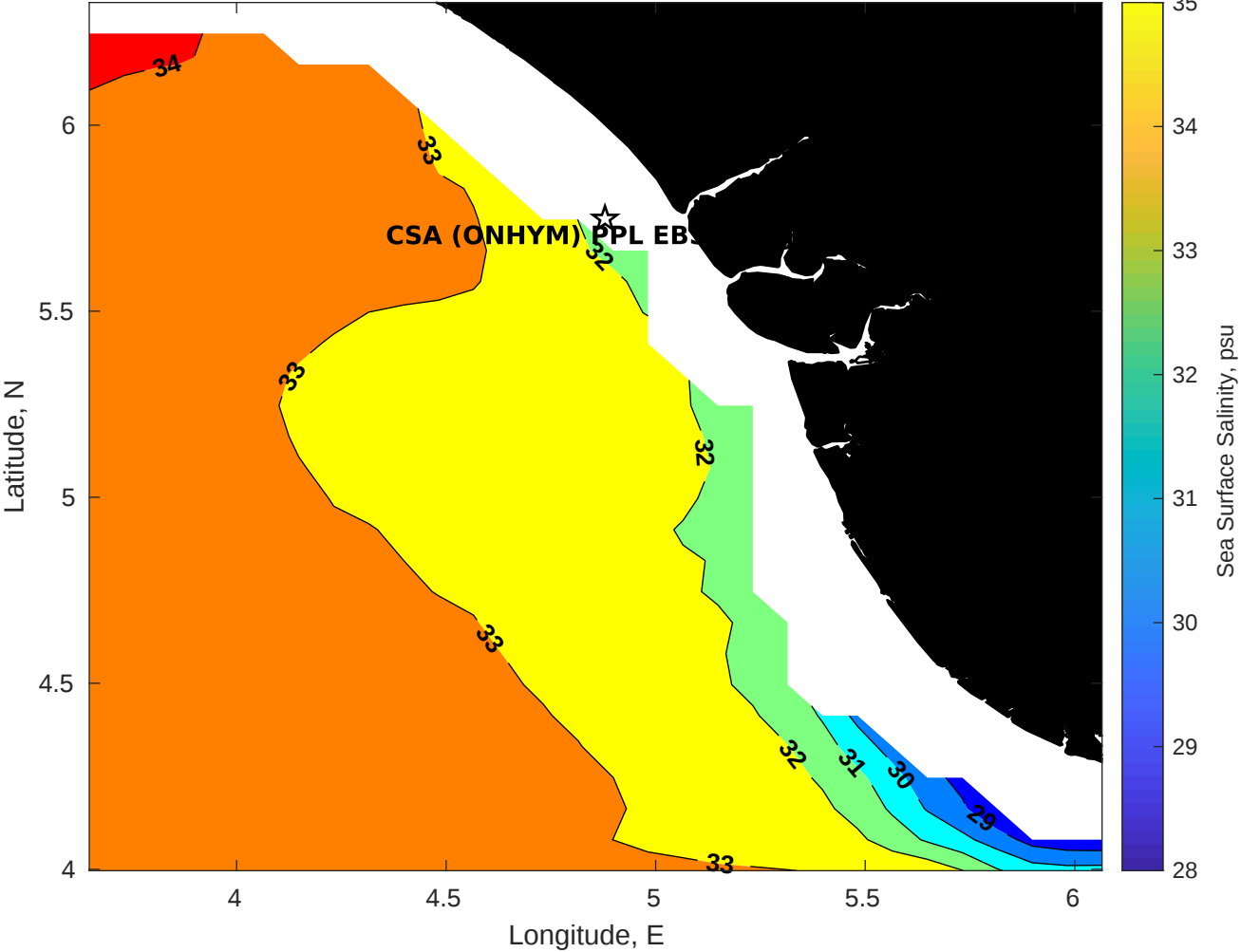
Surface Salinity for CSA (ONHYM) PPL EBS - Nigeria at 06-Nov-2025 00:00:00
