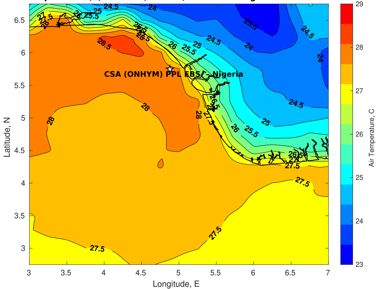
Air Temperature (C) for CSA (ONHYM) PPL EBS - Nigeria at 07-Nov-2025
