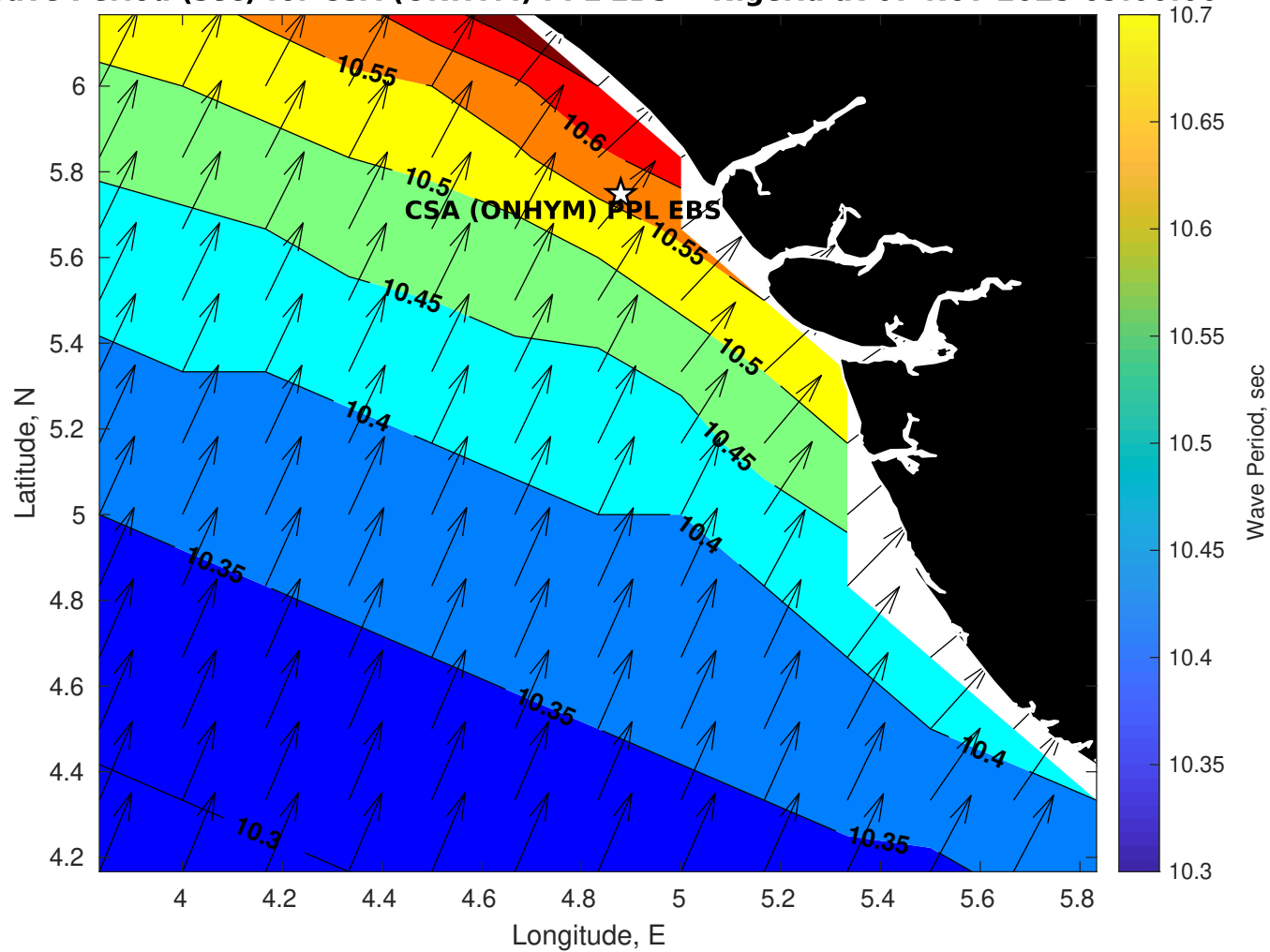
Wave Period (sec) for CSA (ONHYM) PPL EBS - Nigeria at 07-Nov-2025 09:00:00
