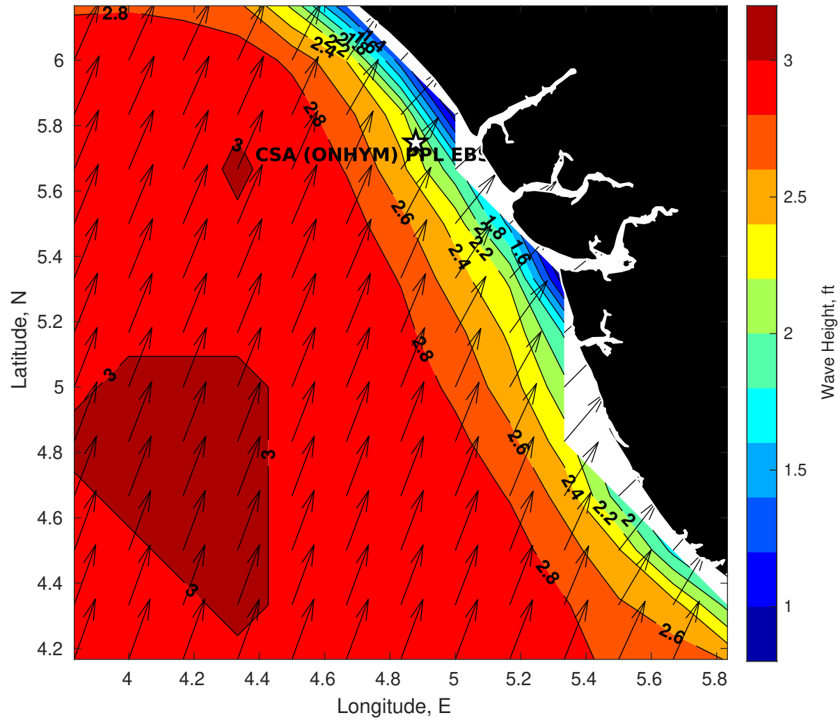
Wave Height (ft) for CSA (ONHYM) PPL EBS - Nigeria at 07-Nov-2025 09:00:00
