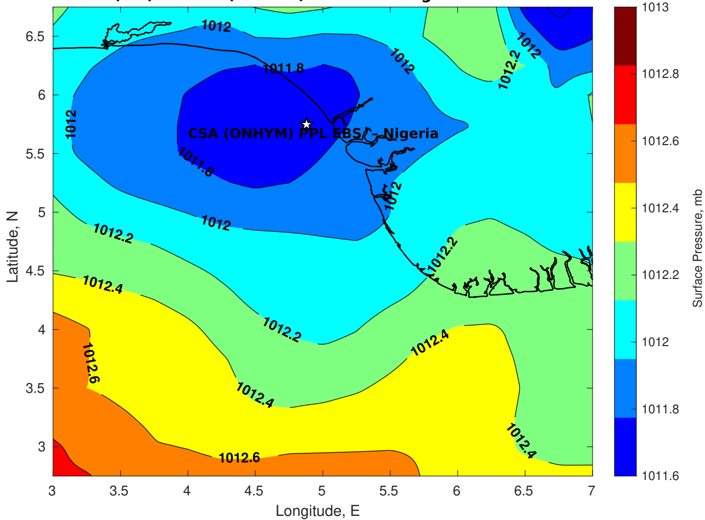
Surface Pressure (mb) for CSA (ONHYM) PPL EBS - Nigeria at 09-Nov-2025 00:00:00
