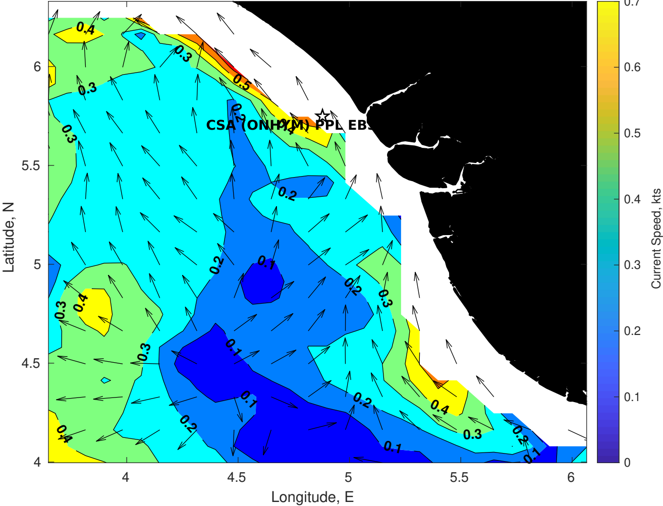
Surface Currents for CSA (ONHYM) PPL EBS - Nigeria at 06-Nov-2025 00:00:00
