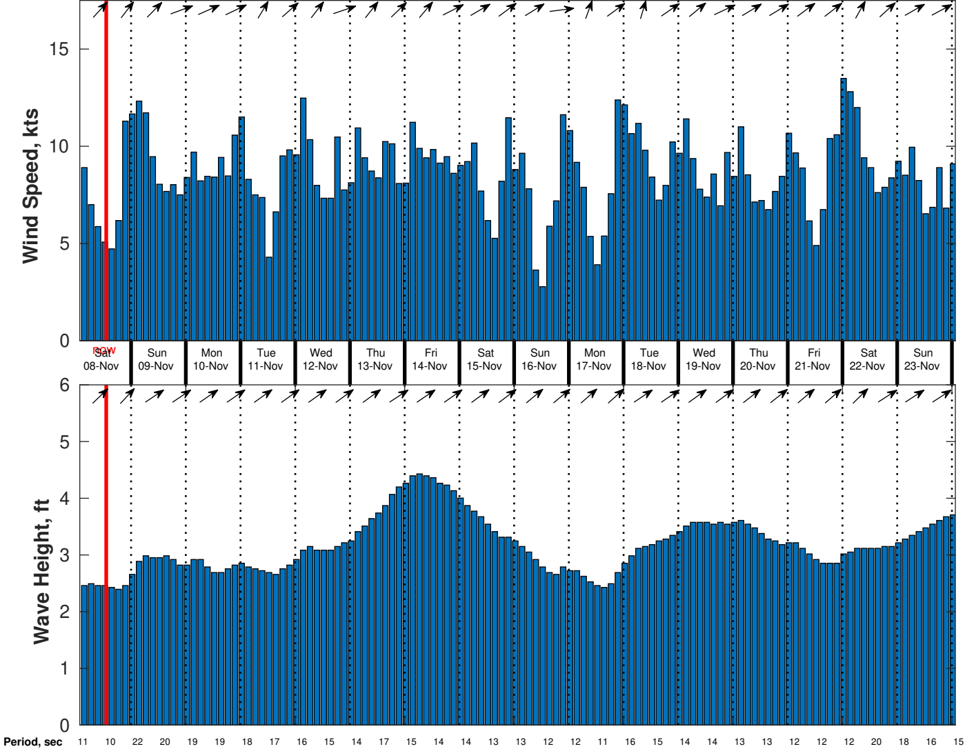
Wind & Wave Forecast for CSA (ONHYM) PPL EBS - Nigeria from 07-Nov-2025 02:00:00 to 23-Nov-2025 02:00:00
