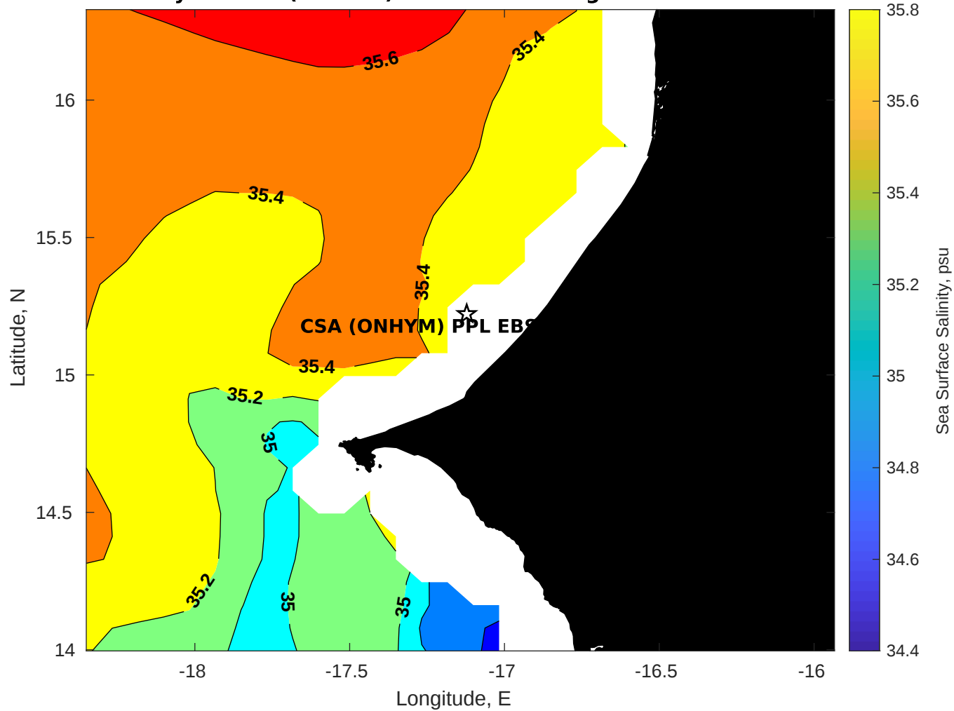
Surface Salinity for CSA (ONHYM) PPL EBS - Senegal at 06-Nov-2025 00:00:00
