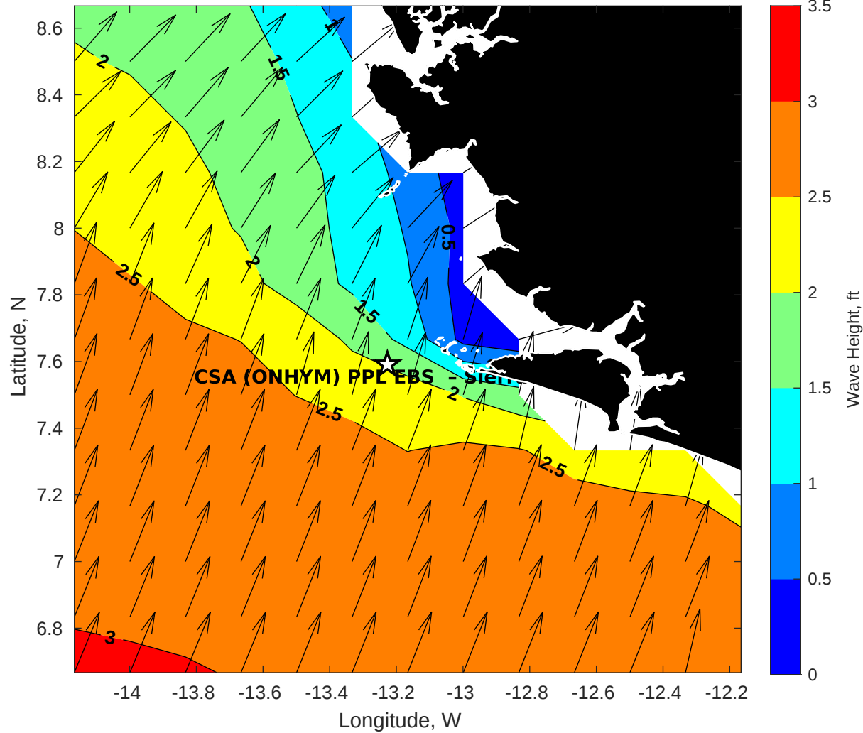
Wave Height (ft) for CSA (ONHYM) PPL EBS - Sierra Leone at 07-Nov-2025 09:00:00
