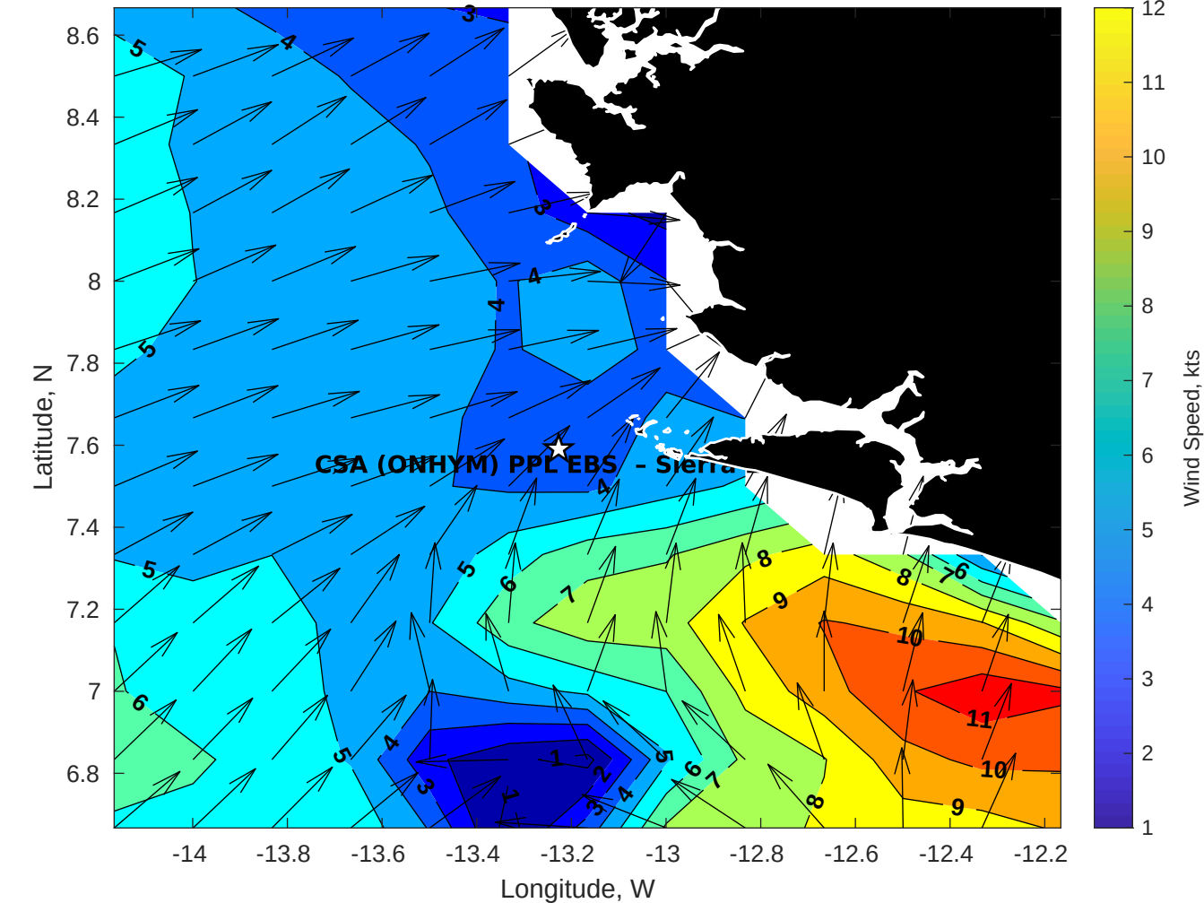
Winds (kts) for CSA (ONHYM) PPL EBS - Sierra Leone at 07-Nov-2025 09:00:00
