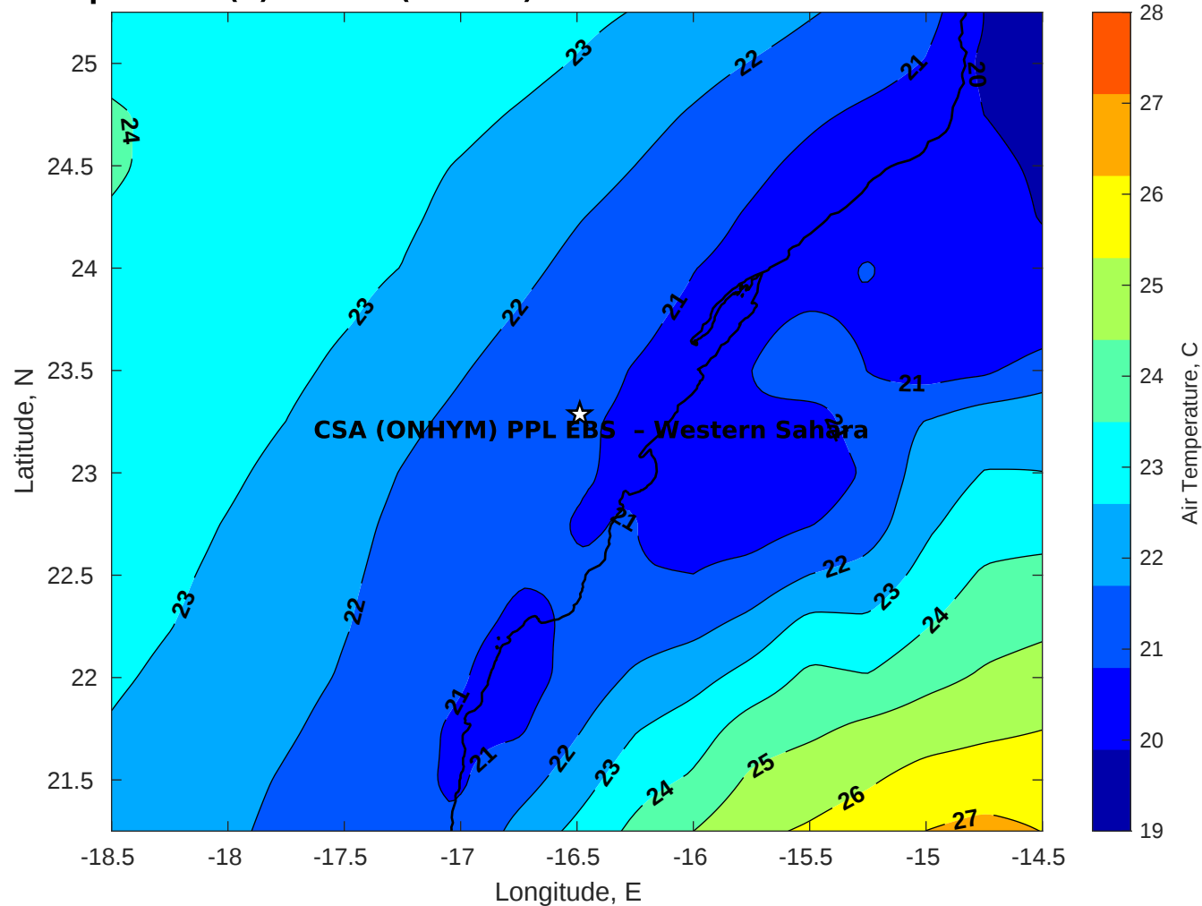
Air Temperature (C) for CSA (ONHYM) PPL EBS - Western Sahara at 07-Nov-2025
