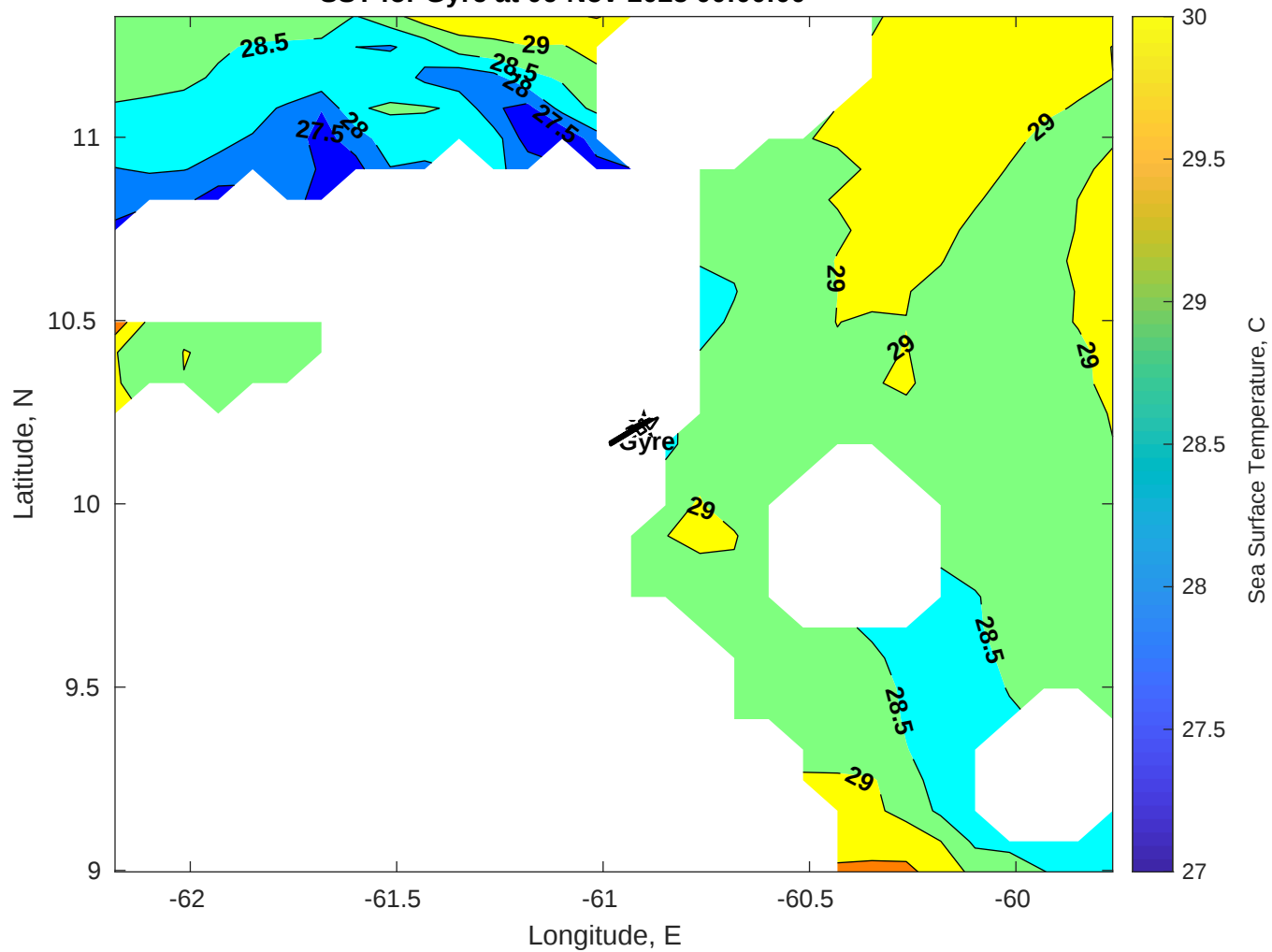
SST for Gyre at 06-Nov-2025 00:00:00
