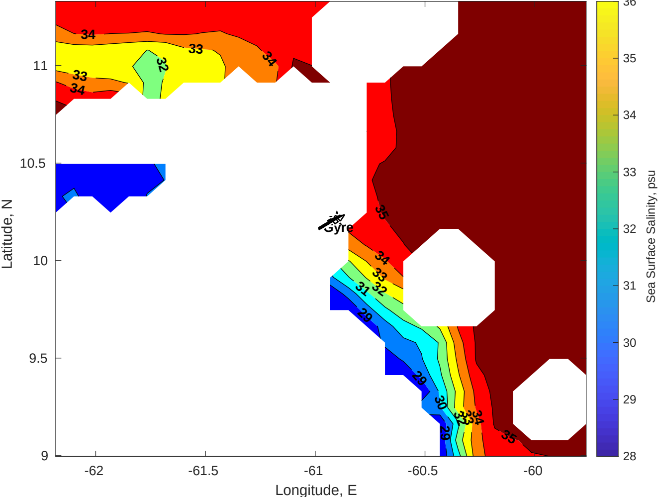
Surface Salinity for Gyre at 06-Nov-2025 00:00:00
