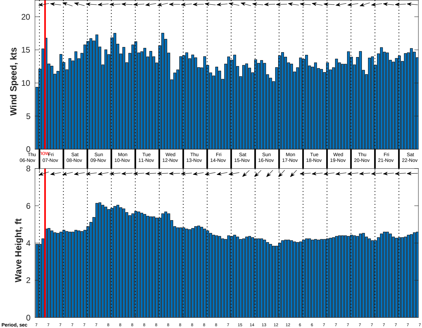
Wind & Wave Forecast for Gyre from 06-Nov-2025 20:00:00 to 22-Nov-2025 20:00:00
